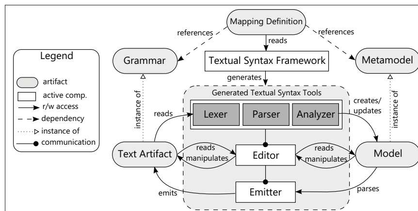
Figure 4.2 General structure of a textual syntax framework
