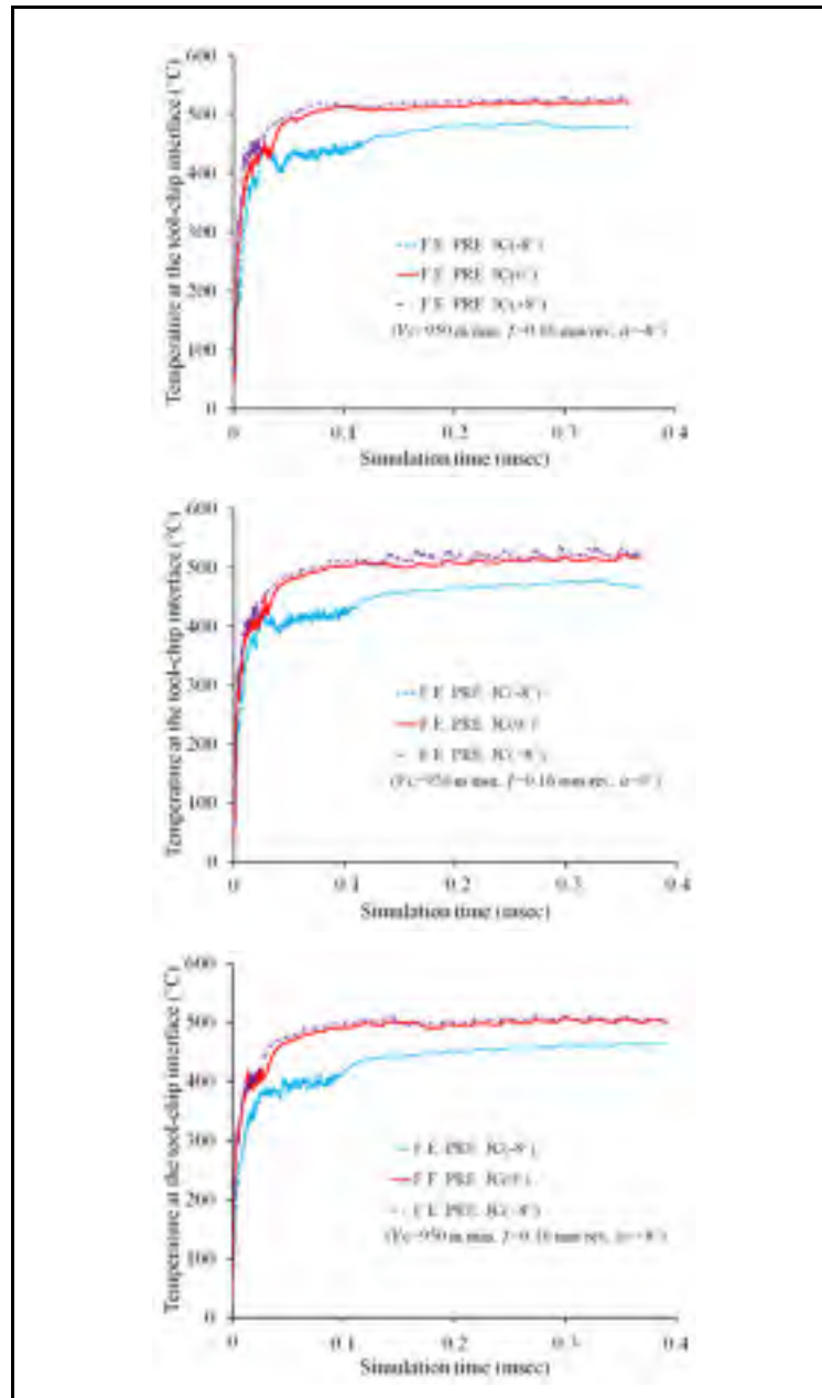
Figure 6-17 Effect of JC sets on temperature at tool-chip interface during cutting
