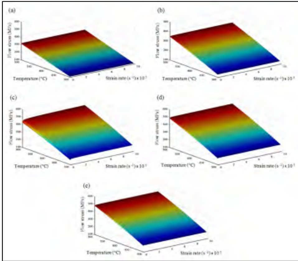
Figure 5-6 Influence of the temperature and strain rate on the material flow stress ( \epsilon=1.5 ) (a) JC(-8°), (b) JC(-5°), (c) JC(0°), (d) JC(+5°), and (e) JC(+8°)
