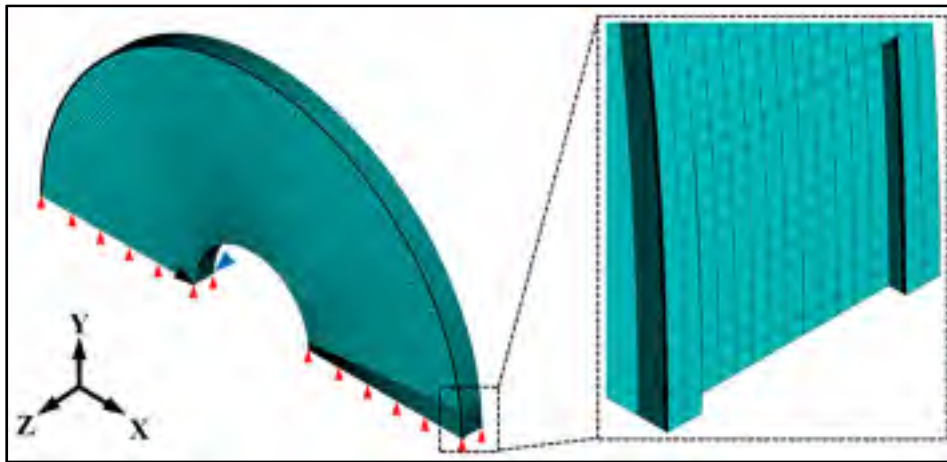
Figure A I-1 Boundary conditions with polishing zone visualization
