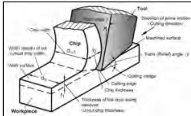
Figure 0-1 Basic terms in orthogonal cutting (Astakhov, 2010)
