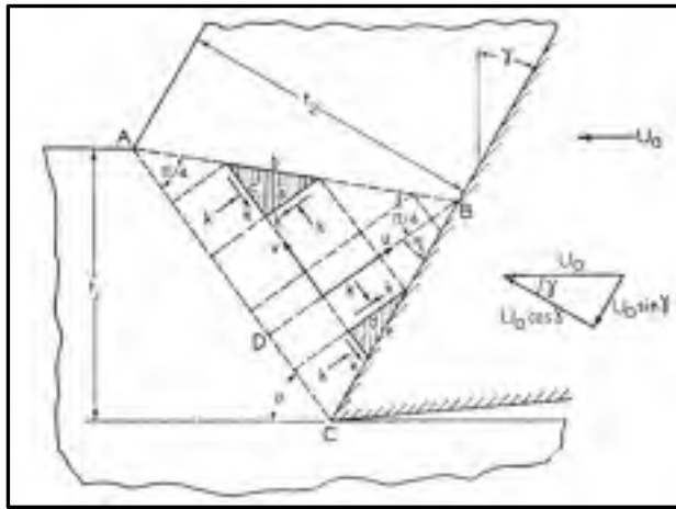
Figure 0-8 Slip line model Adopted from (Lee et Shaffer, 1951)
