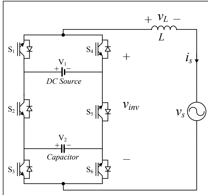
Figure-A II-1 Grid-connected PUC5 inverter
