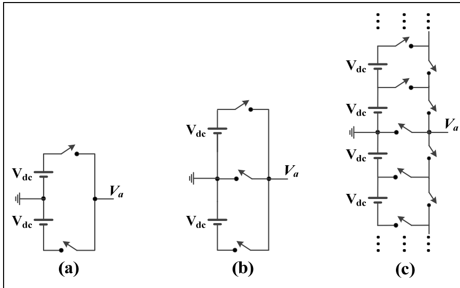
Figure 1.1 One leg of a) 2-level, b) 3-level and c) n-levels inverter
