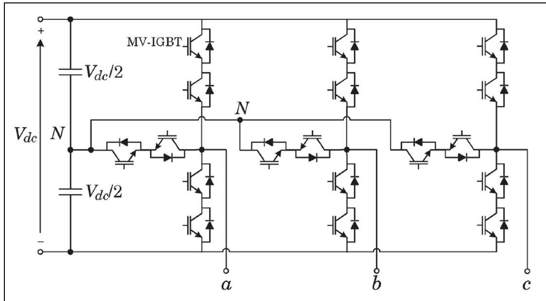
Figure 1.11 3L-NPP
