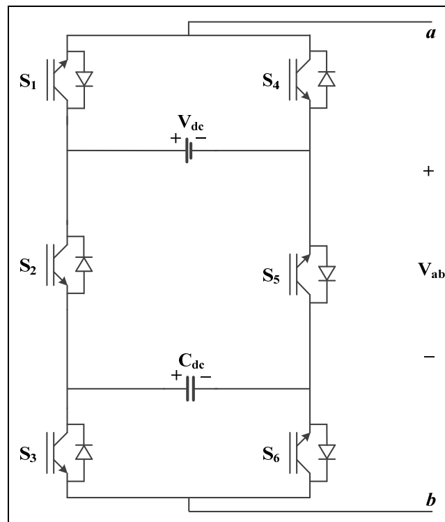
Figure 1.12 Single-Phase 7L-PUC
