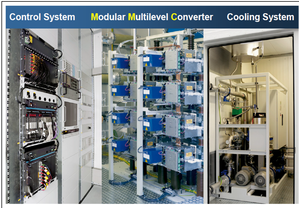
Figure 1.28 MMC for HVDC with its Control System and Cooling System
