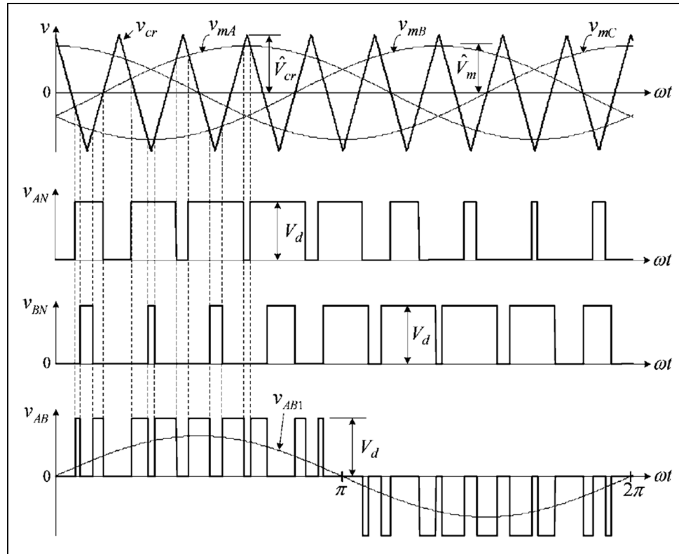
Figure 1.20 Sinusoidal PWM
