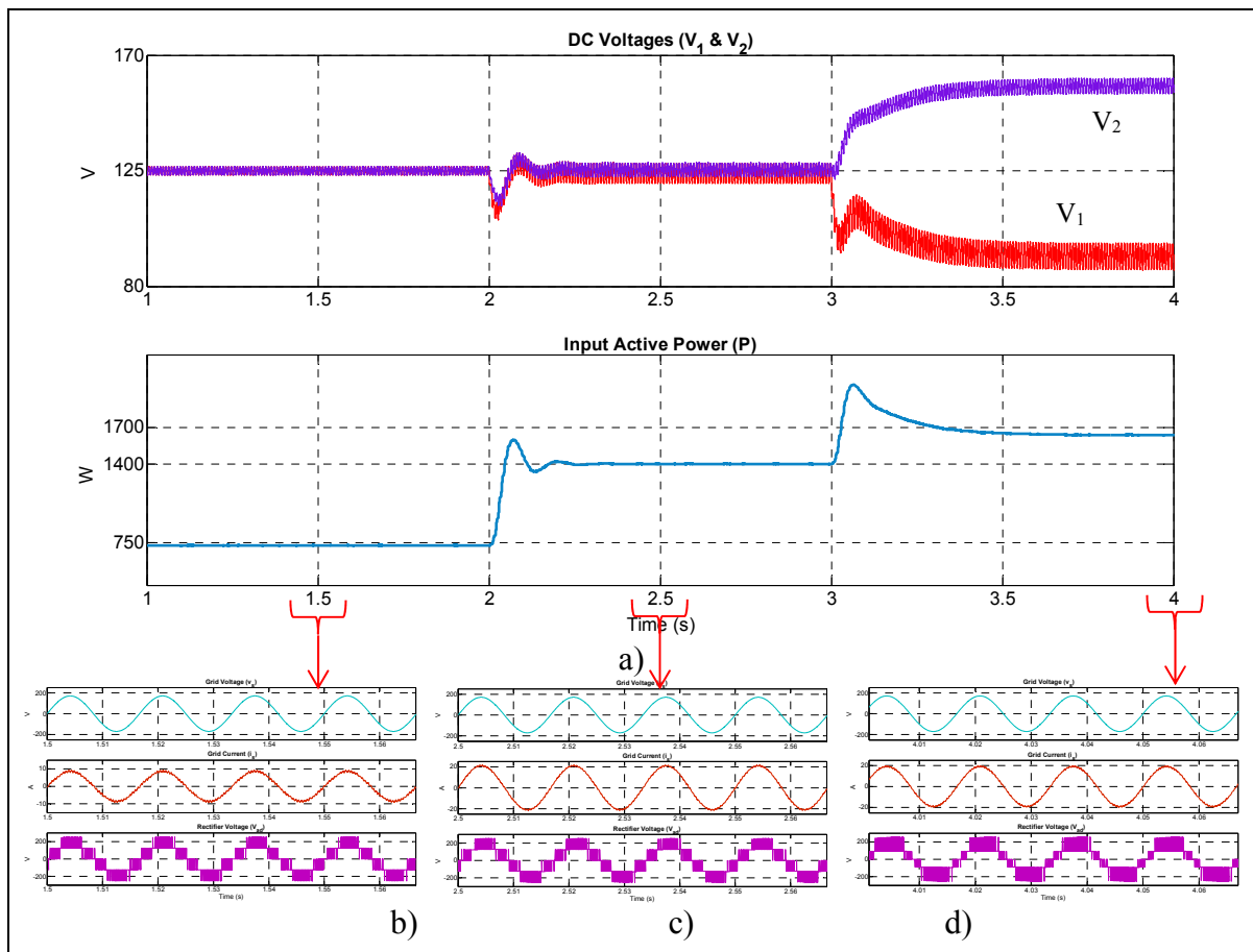
Figure 4.8 Stable and unstable operation of the proposed rectifier
