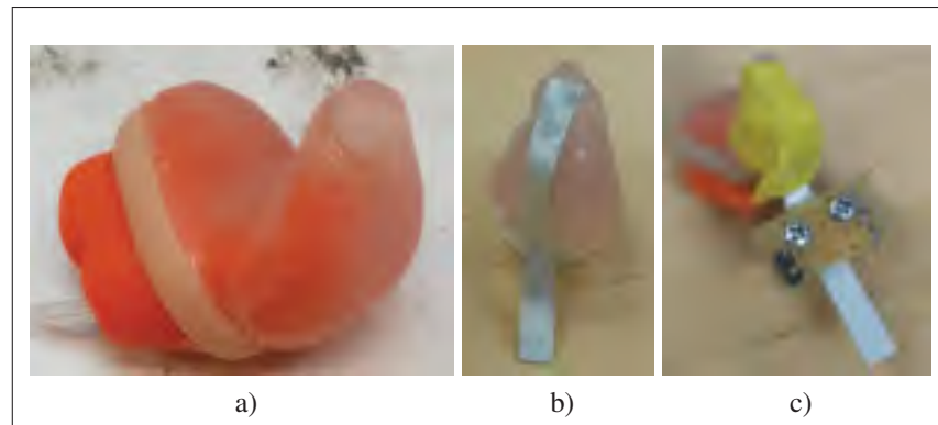
Figure 3.7 a) Custom-fitted earplug obtained using the Sonofit™ instant custom molding pieces, b) Earplug and PVDF strip, and c) Energy harvesting device with connecting terminals
