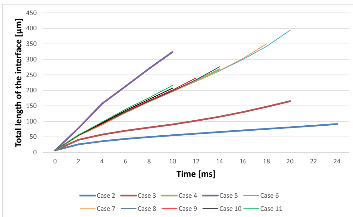
Figure IV-46: Variation of the total length of the interface (μm) in time (ms).
