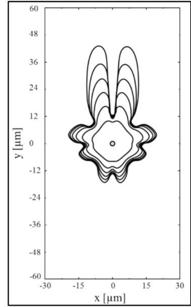
Figure IV-36: Interface evolution of case 9 with T_t = T_m - 18 and T_b = T_m - 6 . Interval time between interfaces is 2 ms.
