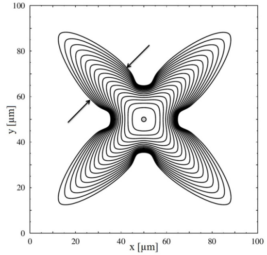
Figure IV-17: Interface evolution of four-fold symmetry. r = 1 \mu\text{m} . \Delta T = 10 \text{ K} . m_\gamma = m_v = 4 . \gamma = 0.05 . \theta_\gamma = \theta_v = \frac{\pi}{4} . Boundary temperature T_\infty - 1 \text{ K} . Interval time between interfaces 1 ms.
