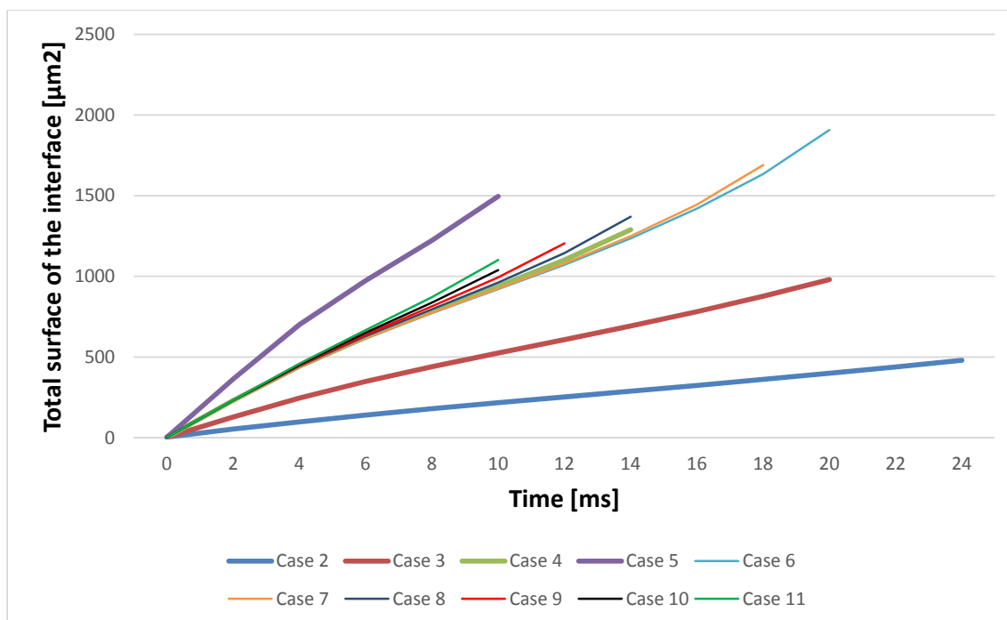
Figure IV-47: Variation of the total surface of the interface (μm²) in time (ms).
