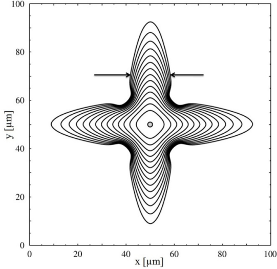
Figure IV-16: Interface evolution of four-fold symmetry. r = 1 \mu\text{m} . \Delta T = 10 \text{ K} . m_\gamma = m_v = 4 . \gamma = 0.05 . \theta_\gamma = \theta_v = \frac{\pi}{2} . Boundary temperature T_\infty - 1 \text{ K} . Interval time between interfaces 1 ms.
