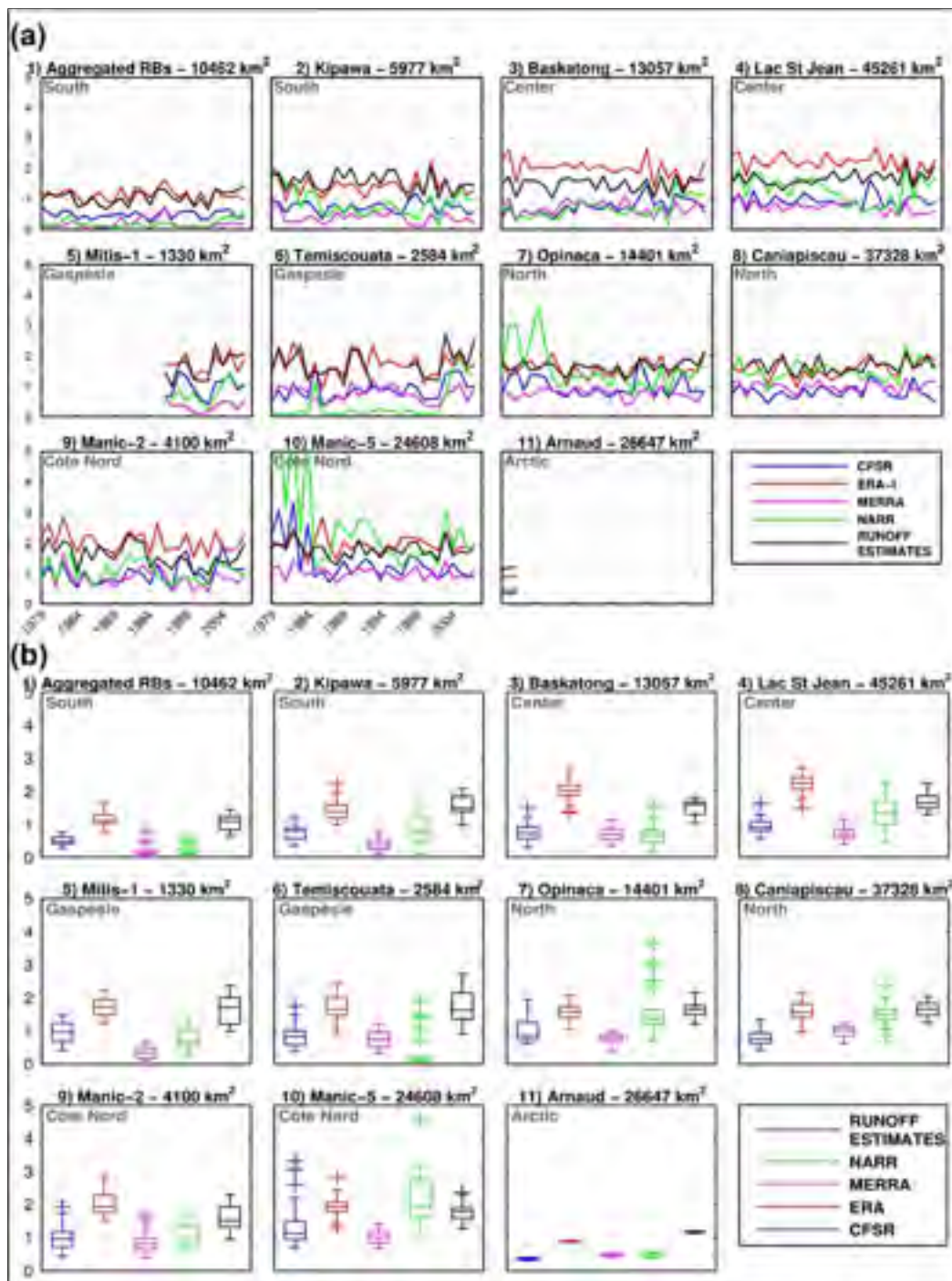
Figure-A I-9 (a) Mean annual runoff (mm day -1 ) from CFSR, ERA-Interim, MERRA, NARR and runoff estimates, from 1979 to 2008 over the eleven selected river basins. Annual time series are limited to the available streamflow observations used to compute the runoff estimates. (b) Distribution of the yearly mean annual runoff (mm day -1 ) from CFSR, ERA-Interim, MERRA, NARR and runoff estimates, from 1979 to 2008 over the eleven selected river basins. The characteristics of the box plots are described in the caption of figure-A I-6
