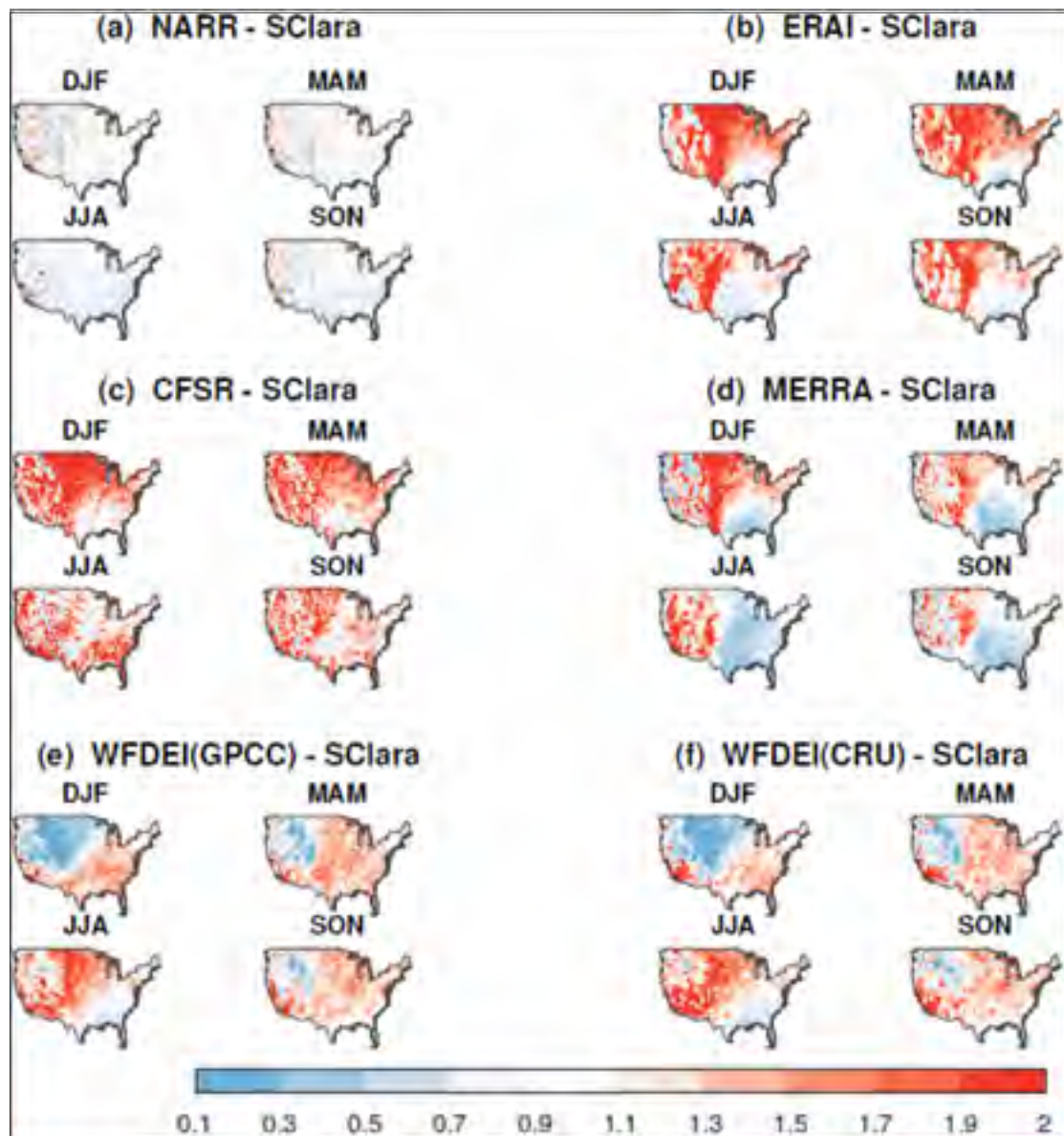
Figure 4.8 Variance ratios of daily precipitation between reanalyses, WFDEI and observed gridded dataset from Santa Clara for each season
