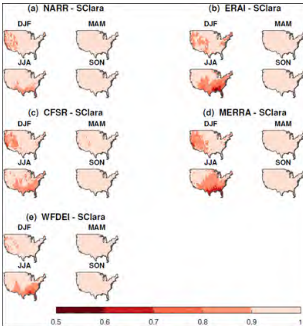
Figure 4.5 Daily temporal correlation between reanalyses, WFDEI and Santa Clara temperature. Results are shown by season and are based on daily data for the 1979–2003 period
