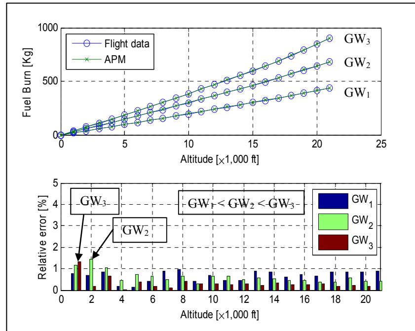
Figure 3.12 Estimated Fuel Burn of Aircraft B in Climb at the highest IAS and for three GW s
