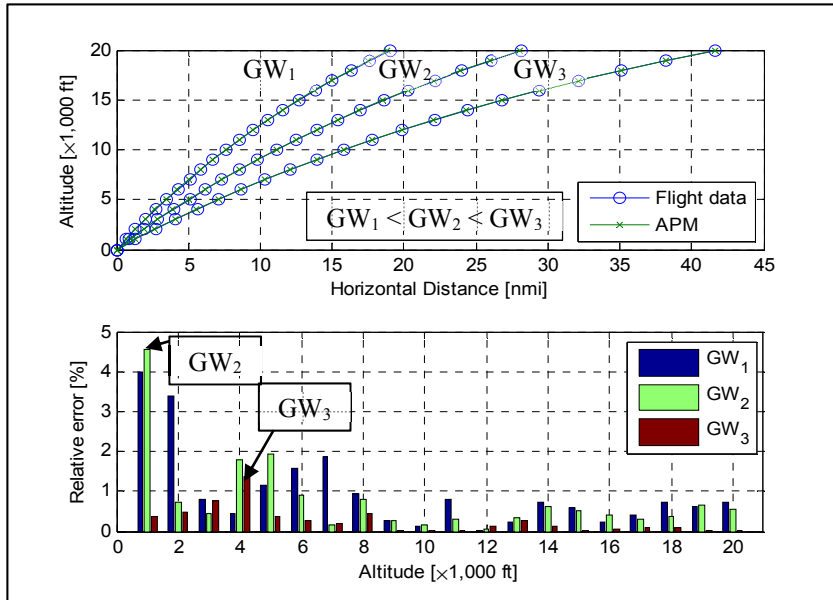
Figure 3.1 Estimated Horizontal Distance of Aircraft A in Climb at the lowest IAS and for three GWs
