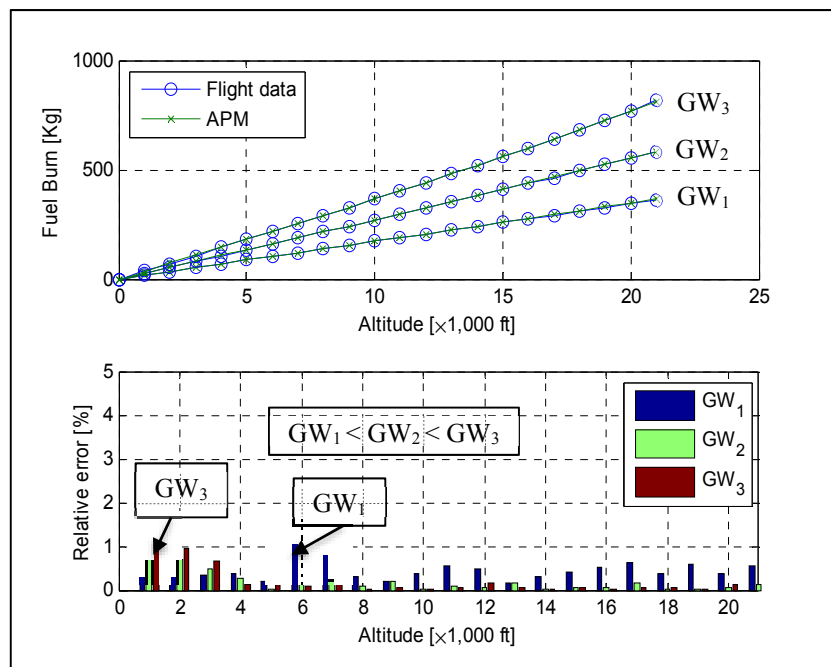
Figure 3.10 Estimated Fuel Burn of Aircraft B in Climb at a middle IAS and for three GWs
