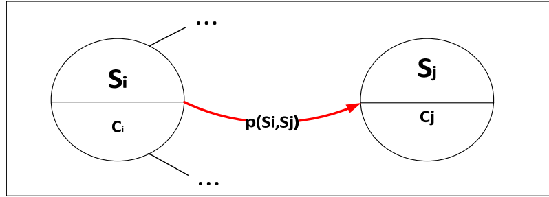
Figure 5.4 state transition probability
