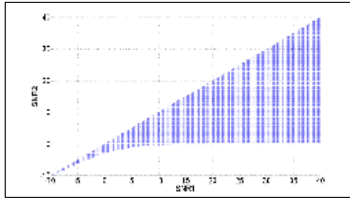
Figure 4.6 Values of SNR_1 and SNR_2 that satisfy C_1 + C_{2c} \geq C_1 (waterfilling)
