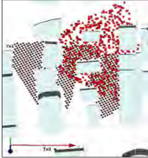
Figure 2.12 Setup 3 and 4 (Tx1/Tx2 center left/bottom)
