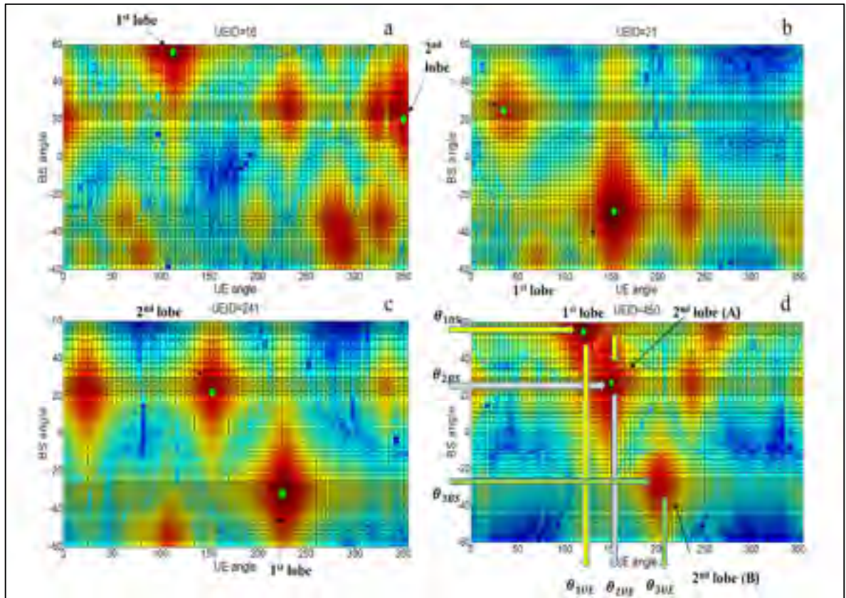
Figure-A VIII-1 Power lobes for different UEs
