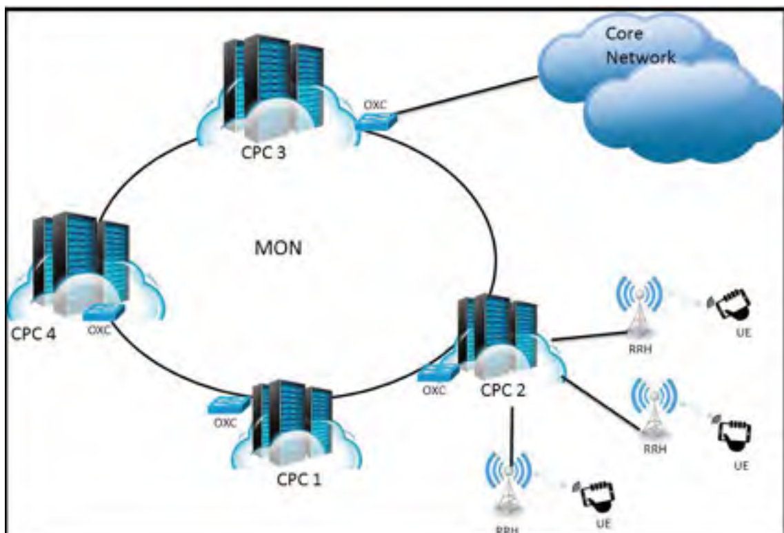
Figure 1.5 Architecture CVN
