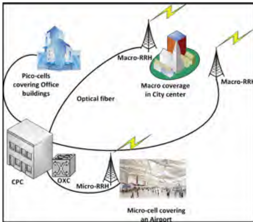
Figure 1.6 Architecture RVN
