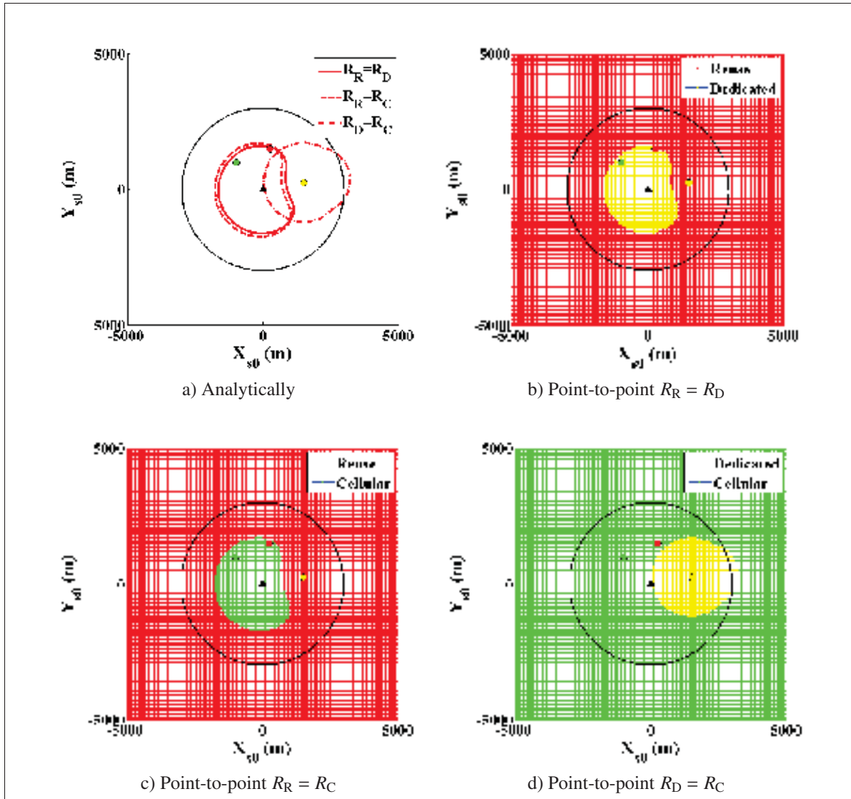
Figure 1.5 Comparison of equireate boundaries derived analytically and from point-to-point simulation approaches, when UE_s moves in the network and the communication channels are modeled as LoS pathloss
