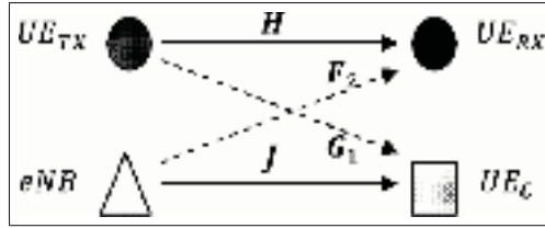
Figure-A I-3 MIMO interference channel in reuse mode
