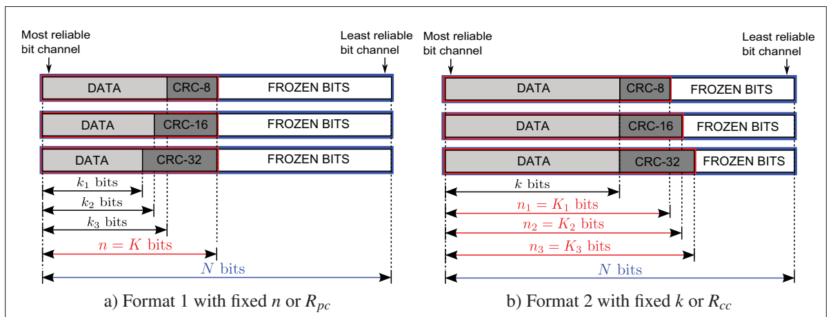
Figure 3.8 Bit-arrangement formats
