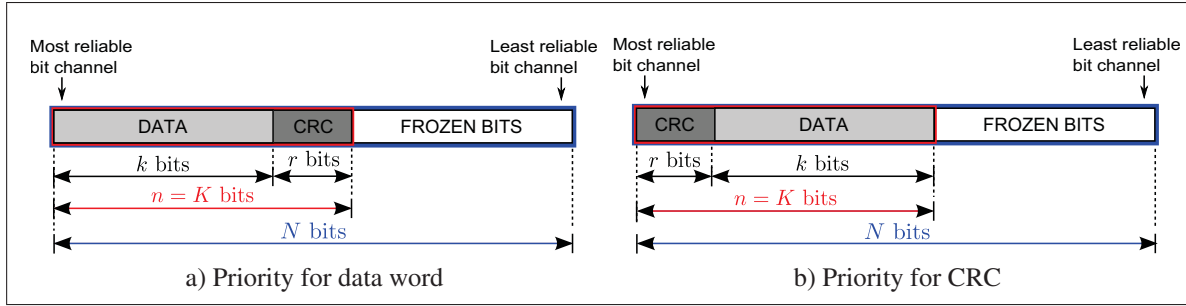
Figure 3.6 Assignment of bit channels in polar codeword
