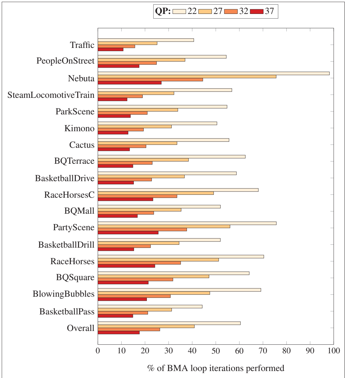
Figure 5.11 Sequence-wise results for the percentage of iterations performed by the block-matching loop in the proposed solution. A value of 100% indicates that all the iterations of the loop are performed.
