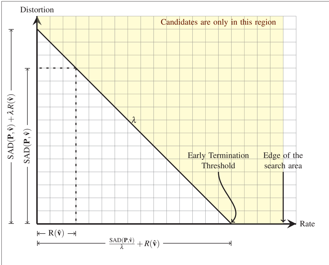
Figure 5.3 Geometric representation of the early termination threshold.
