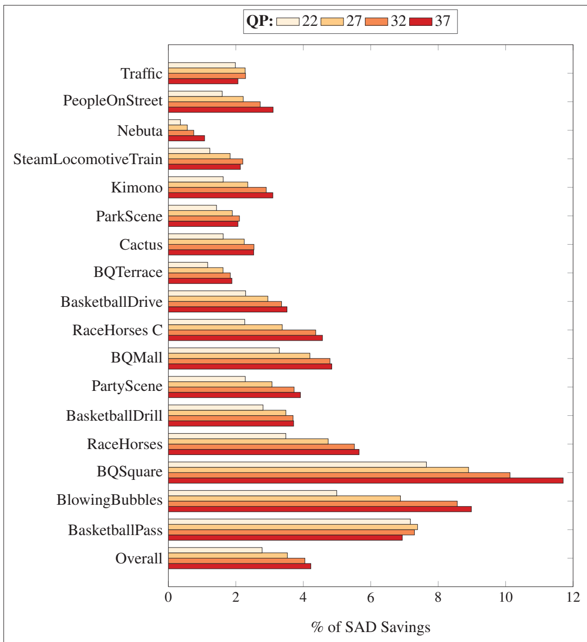
Figure 5.9 Percentage of SAD operation savings, per sequence, for HM-CBSEA, when compared to HM-RCSEA, for the main profile and RA settings.
