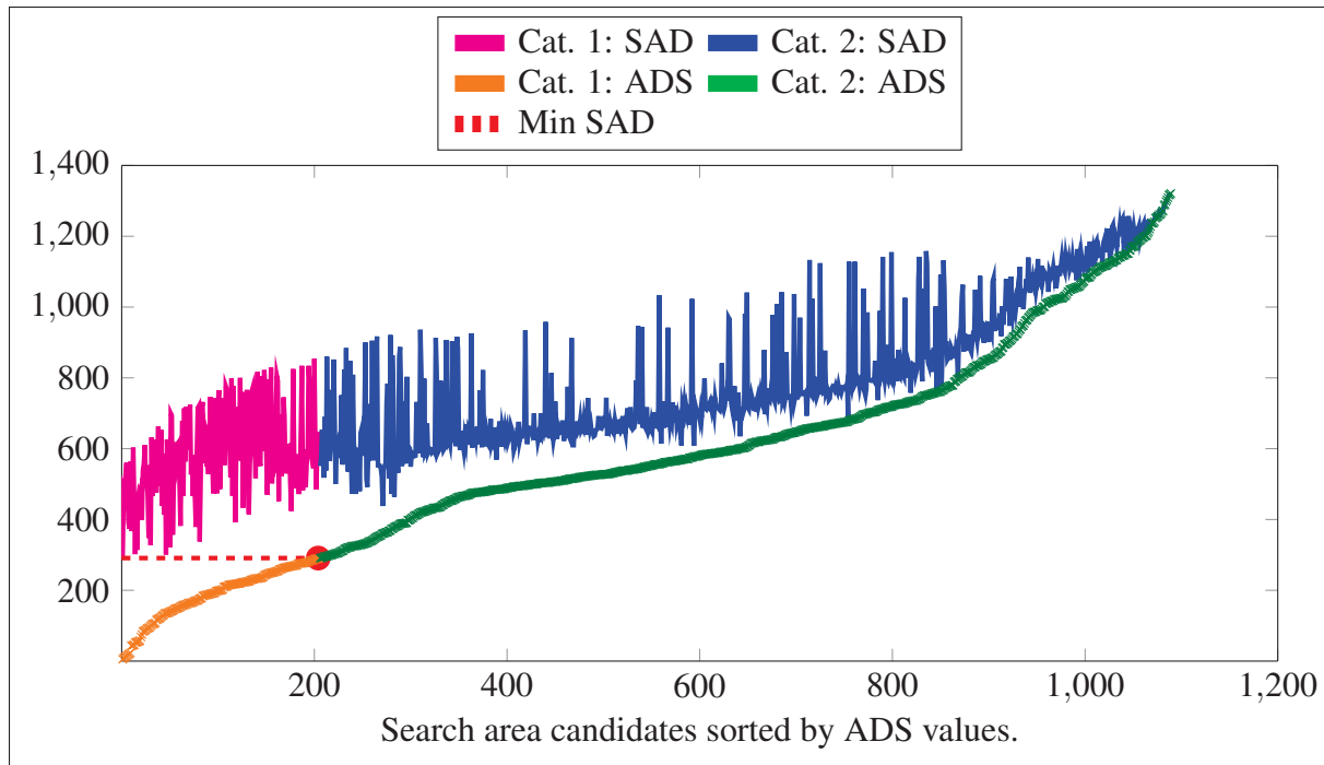
Figure 5.1 SAD and ADS values of category 1 and category 2 candidates. Adapted from Trudeau et al. (2015a)
