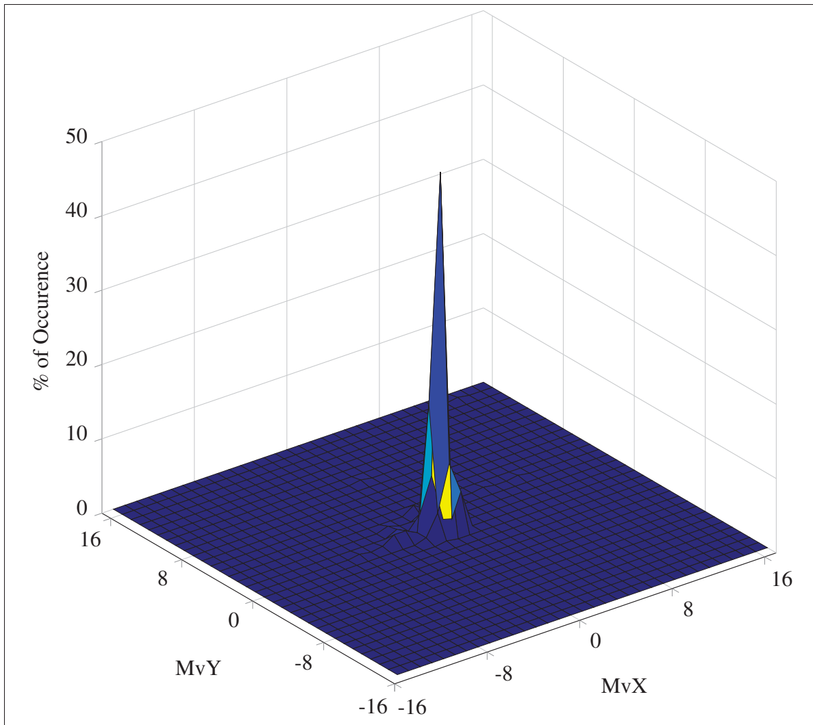
Figure 4.2 Example of the distribution of the position of the global minimum inside the search area for a quasi-stationary frame. Global minimums are distributed at the center of the search area.
