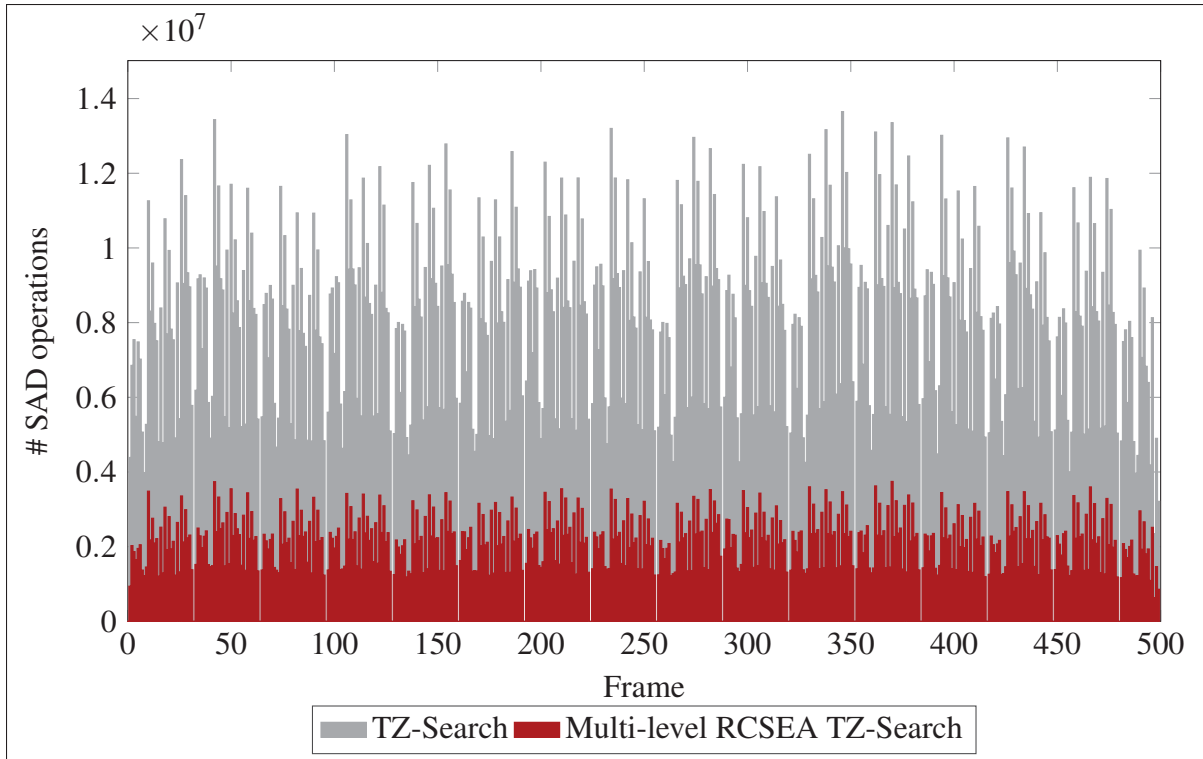
Figure 7.6 Comparison of the number of SAD operations performed by TZ-search with and without ML-RCSEA for the BasketballDrill sequence, QP=22 and using the LD Main profile.
