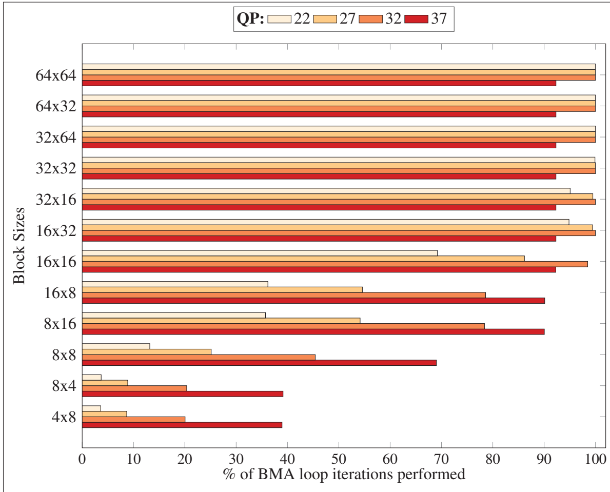
Figure 5.12 Block-wise results for the percentage of iterations performed by the block-matching loop in the proposed solution. A value of 100% indicates that all the iterations of the loop are performed.
