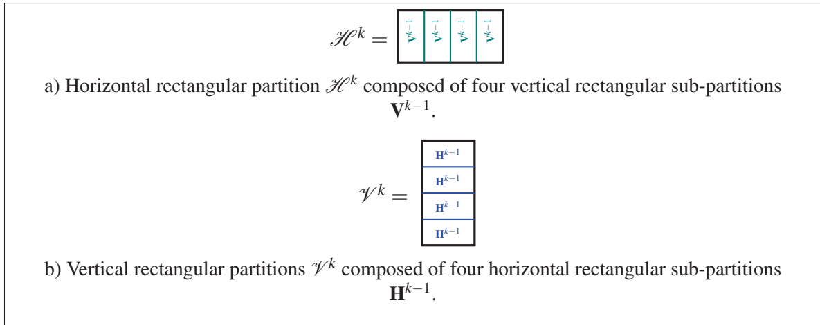
Figure 7.2 Proposed multi-level composition pattern for rectangular partitions.
