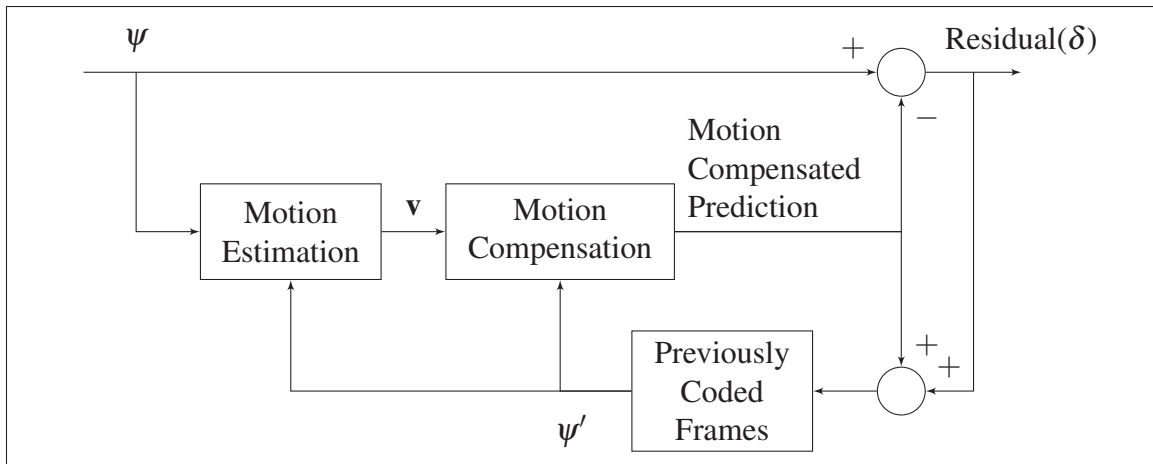
Figure 2.1 Generic outline of temporal prediction in a block-based hybrid video encoder
