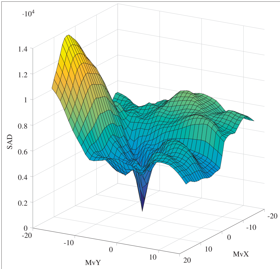
Figure 4.1 Example of the surface of the error criterion over the search area. This surface is not monotonically decreasing towards the global minimum.
