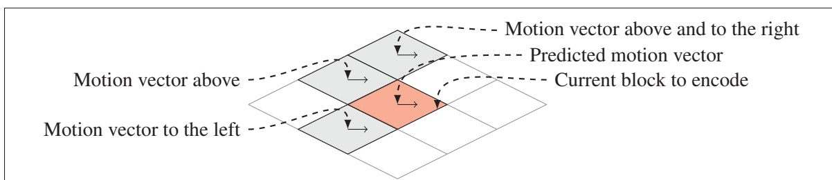
Figure 2.5 In AVC, the predicted motion vector is the median of the motion vectors: to the left, above and above and to the right of the current block
