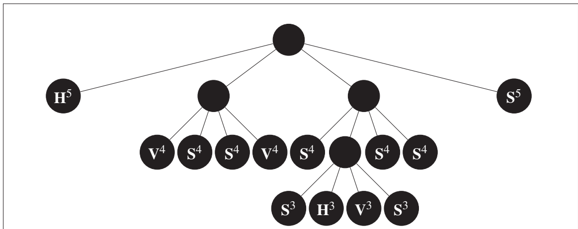
Figure 1.2 Example of a quad-tree decomposition and block partitioning. The corresponding blocks and partitions are shown in Figure 1.3
