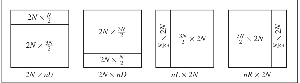
Figure 1.4 Asymmetric partitioning used in HEVC.
