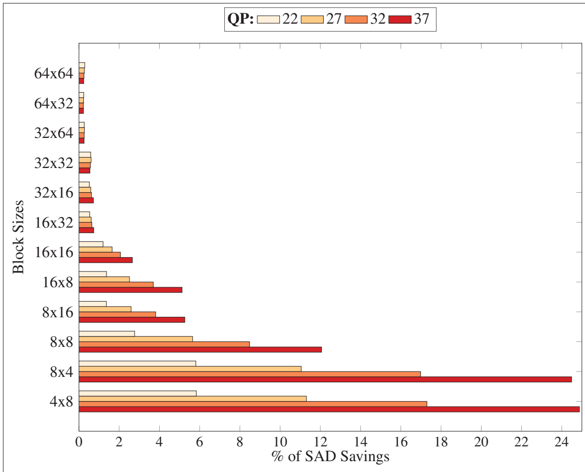
Figure 5.10 Percentage of SAD operation savings, per block size, for HM-CBSEA, when compared to HM-RCSEA, for the main profile and RA settings.
