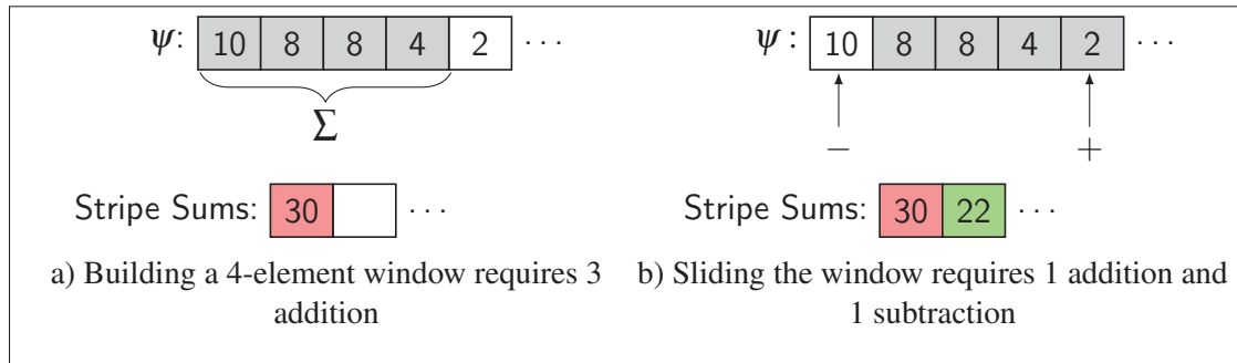
Figure 3.2 Example of the first pass of the sliding window approach proposed by Li and Salari. This data will be reused in fig. 3.3 to sum 4 \times 4 blocks
