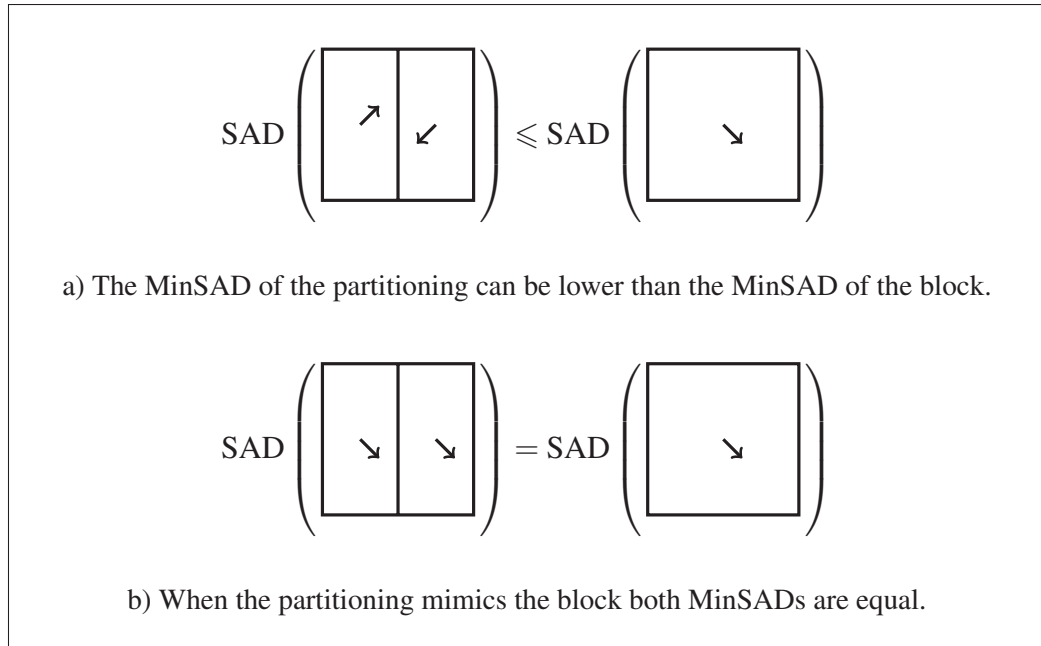
Figure 6.1 Visualization of LowSAD, a lower bound for blocks that is based on the reuse of MinSADs from their partitioning.
