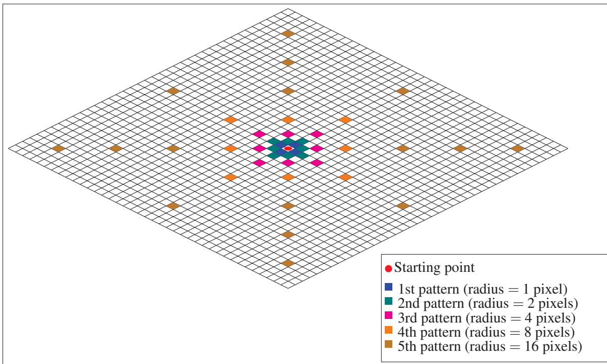
Figure 4.4 Arrangement of patterns of exponentially increasing sizes used by TZ-Search to evaluate a starting point.
