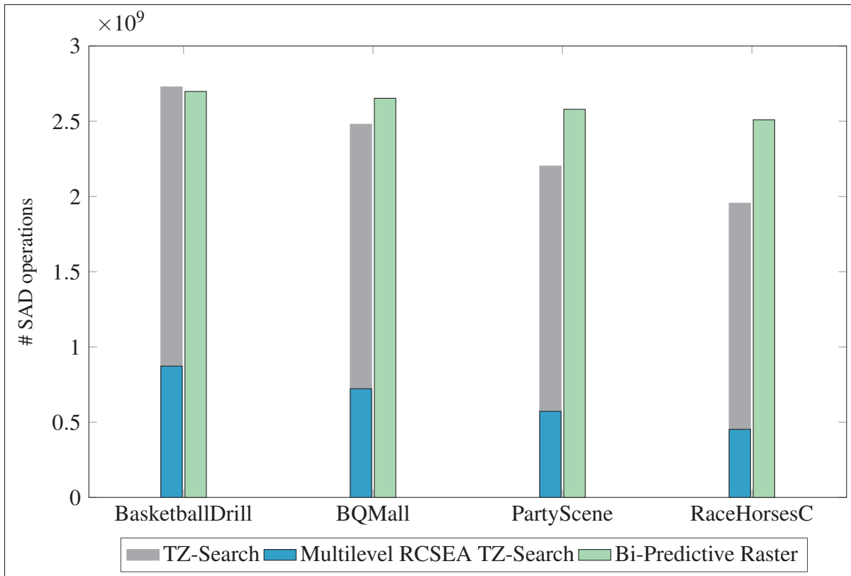
Figure 7.5 Comparison of the number of SAD operations performed by the HM. After introducing ML-RCSEA, bi-predictive raster refinement now becomes the predominant source of SAD operations.
