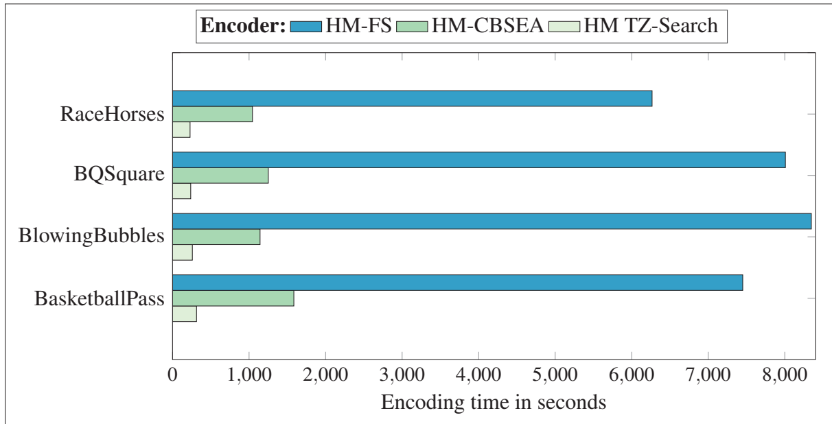
Figure 5.13 Encoding time in seconds, for version 3, when compared to HM TZ-Search, for class D sequences using the main profile and RA settings.
