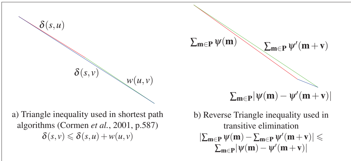
Figure 3.1 Geometric example of the triangle inequality and the reverse triangle inequality with regards to shortest path algorithms and transitive elimination
