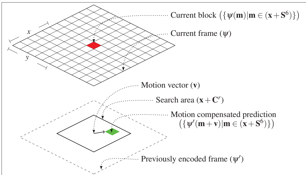
Figure 2.2 Elements and notations of motion estimation and motion compensation
