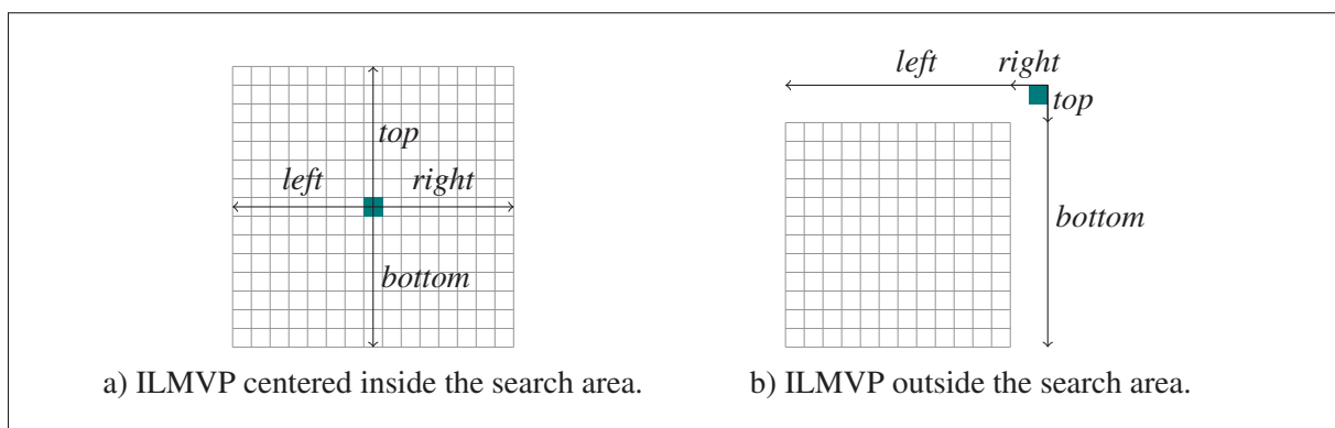
Figure 5.7 Search area defined by: top , bottom , left , right . The colored candidate is the ILMVP. In fig. 5.7b, the ILMVP is outside the search area and the values of top and right are negative.
