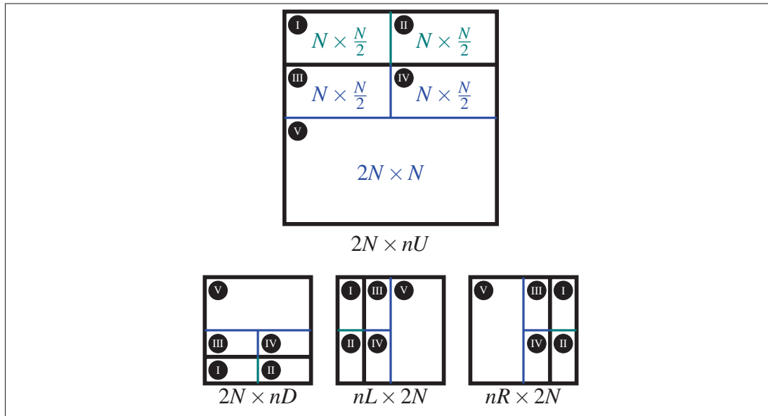
Figure 7.4 Proposed multi-level composition pattern to perform ML-RCSEA on an asymmetric partitioning using pre-computed symmetric sub-partitions.
