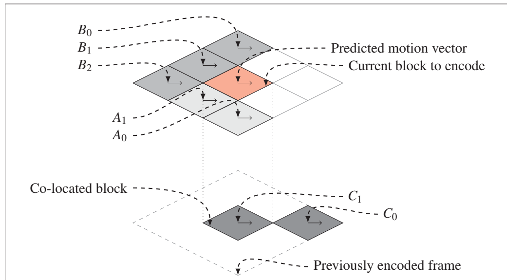
Figure 2.6 In HEVC, the predicted motion vector is signaled from a list of candidates. This list contains up to two spatial candidates ( a \in \{A_0, A_1\}, b \in \{B_0, B_1, B_2\} ) and one temporal candidate ( c \in \{C_0, C_1\} )
