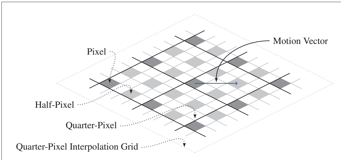
Figure 2.3 Example of a half-pixel motion vector in a quarter-pixel accuracy grid of samples. Half-pixel and quarter-pixel samples are interpolated from integer pixel values
