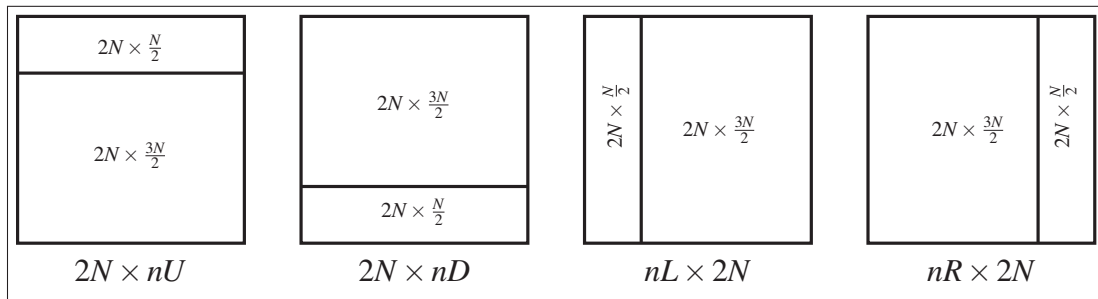
Figure 7.3 AMP used in HEVC. Multiple new partition sizes must be considered. Some partitions are offset and others overlap each other. These are all issues for ML-RCSEA.
