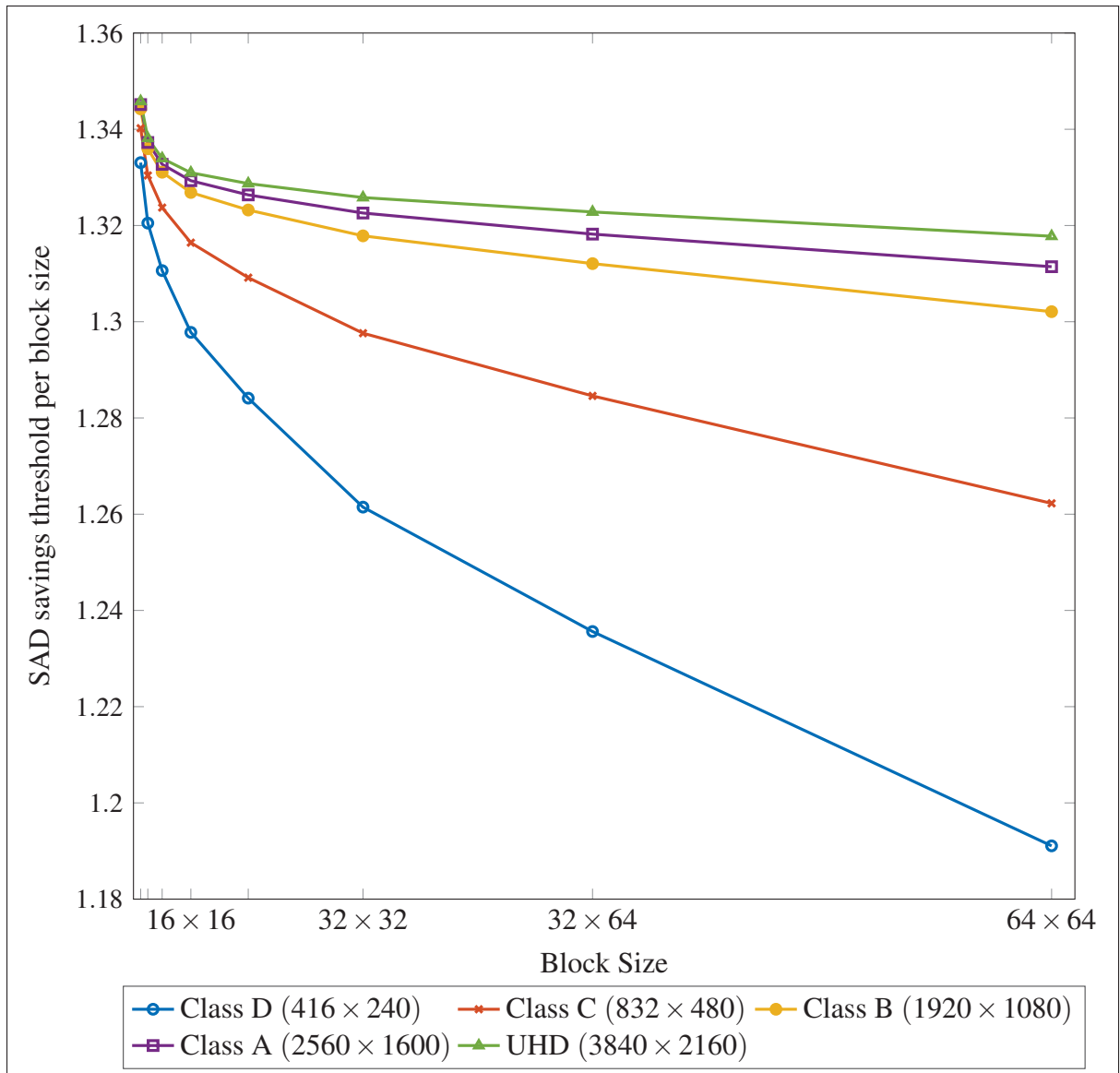
Figure 7.1 SAD savings threshold per block for HEVC block/partition sizes and for common frame resolutions.
