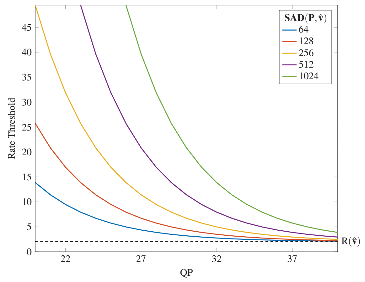
Figure 6.2 Relationship between the rate threshold and \text{SAD}(\mathbf{P}, \hat{\mathbf{v}}) over the recommended range of QPs for HEVC.
