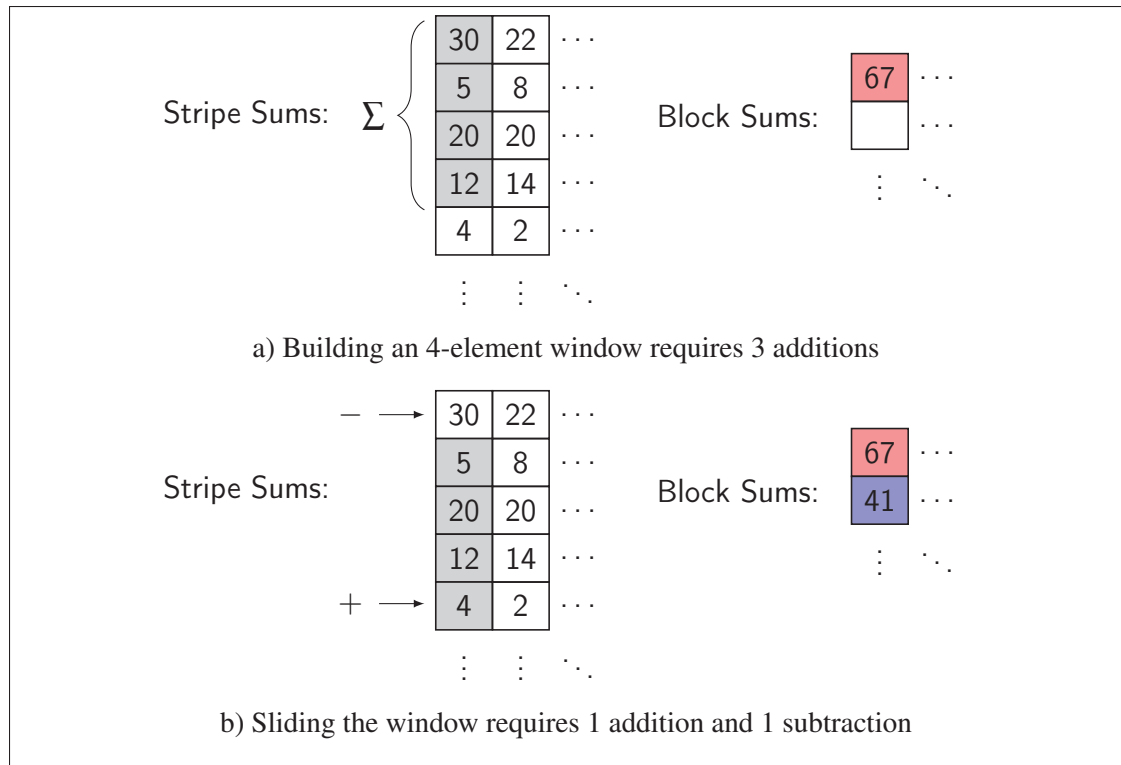
Figure 3.3 Example of the second pass of the sliding window approach proposed by Li and Salari. The stripes used where in part computed in fig. 3.2.
