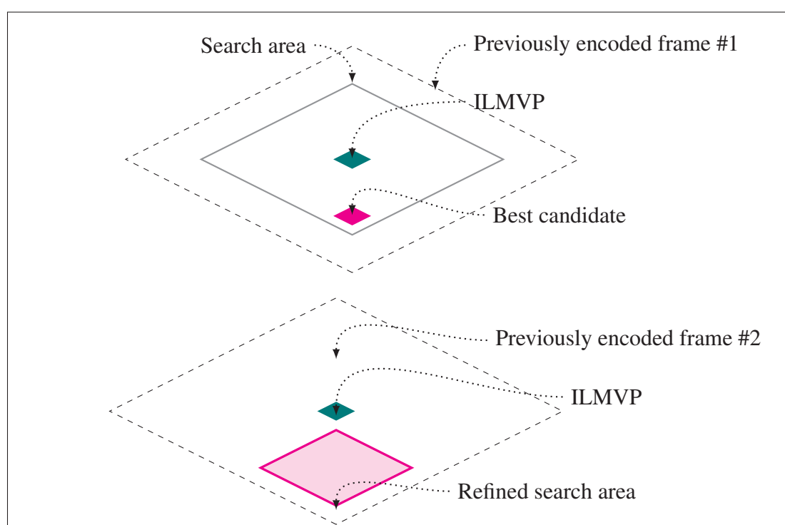
Figure 5.6 Two-step approach used in modern encoders for fractional pixel accuracy search, notice that the ILMVP (teal block) is not in the refined search area (magenta surface).
