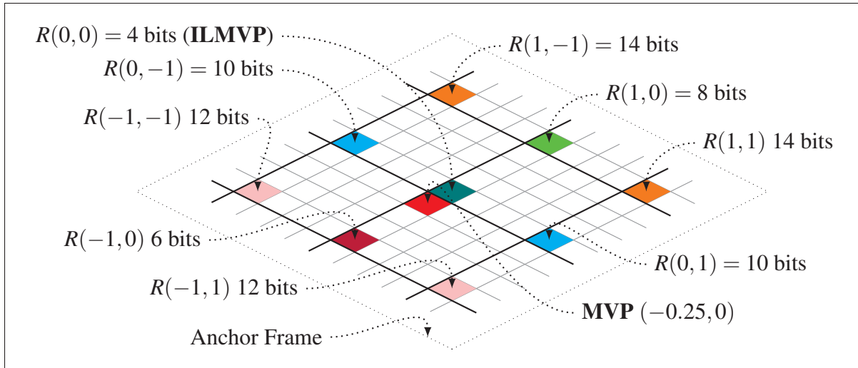
Figure 5.5 The MVP is shown with a red block at (-0.25, 0) . The candidates are symmetrically located around the ILMVP (teal block); however, horizontal integer level candidates on the left require fewer bits than the candidates on the right.
