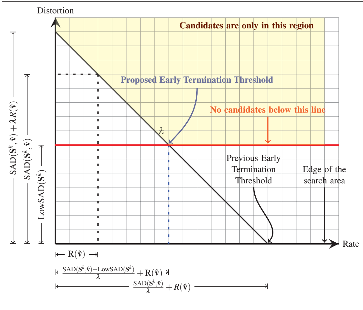
Figure 6.3 Geometric representation of the early termination thresholds.
