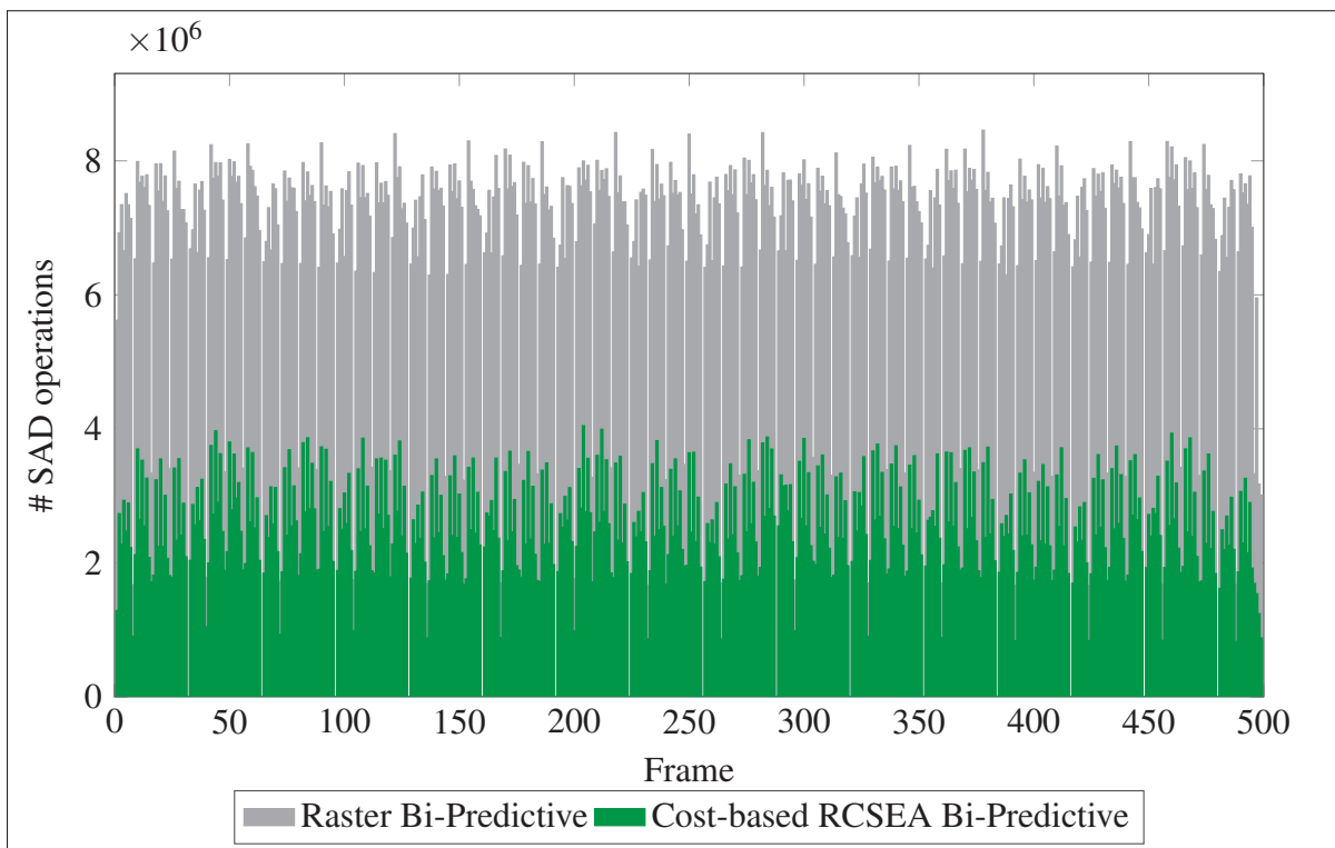
Figure 7.7 Comparison of the number of SAD operations performed by bi-predictive raster refinement compared with a cost-based RCSEA refinement for the BasketballDrill sequence, QP=22 and using the LD Main profile.
