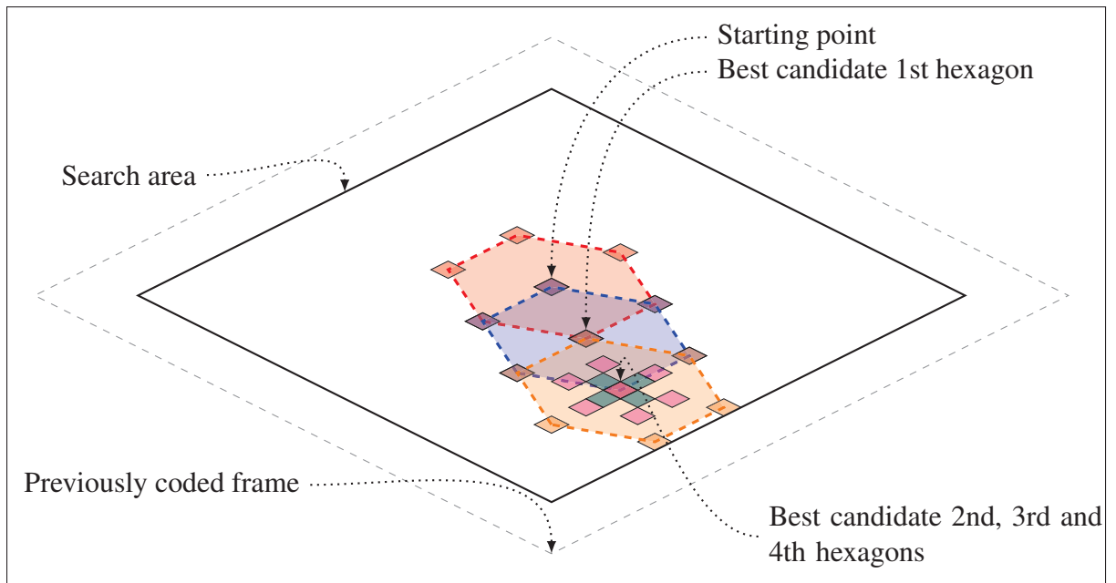
Figure 4.3 Example of a 2-D-logarithmic search algorithm using a combination of an hexagon and a cross pattern. First, the hexagon is used until it converges, then a cross is used as a refinement.
