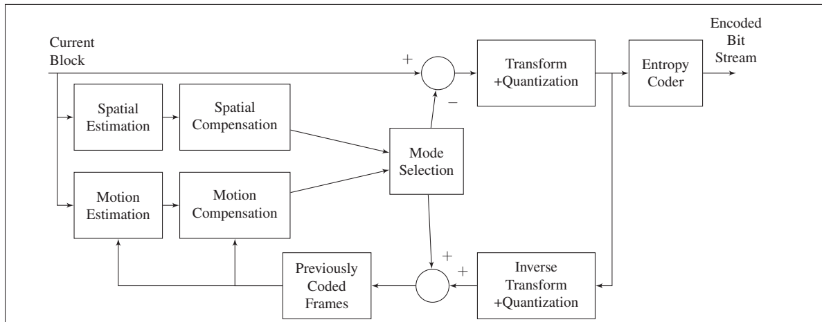
Figure 1.1 Generic outline of the design of a block-based hybrid video encoder
