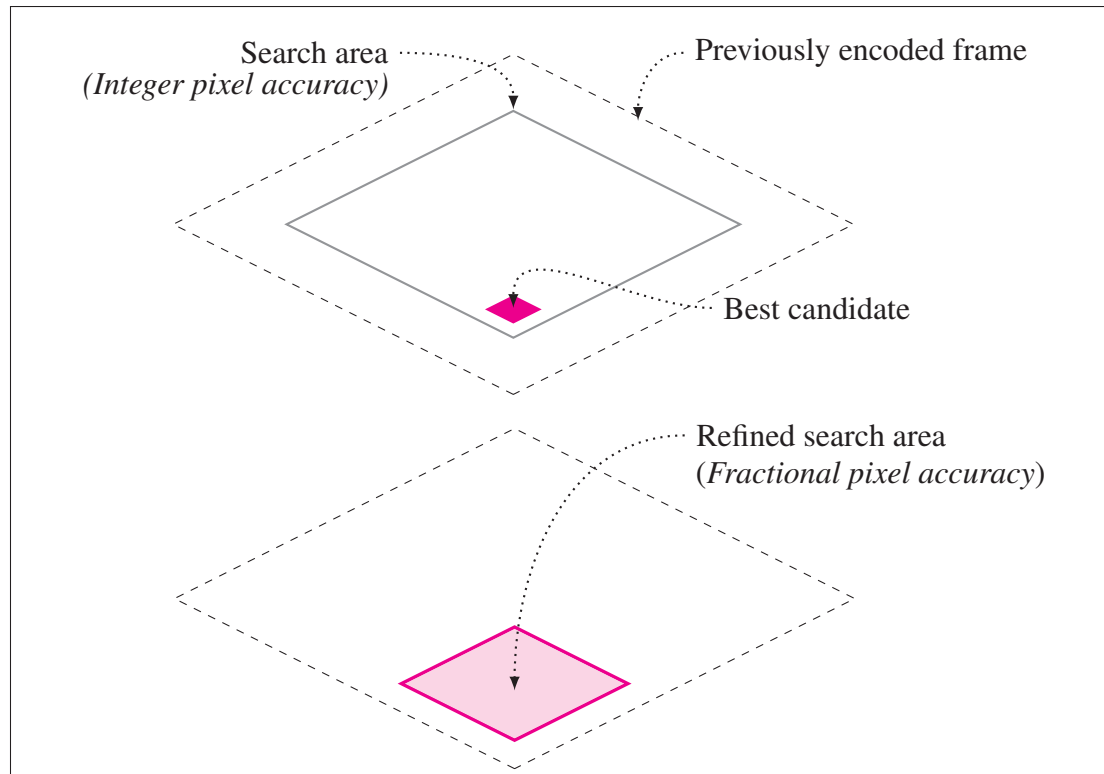
Figure 2.4 Two-step approach used in modern encoders for fractional pixel accuracy search
