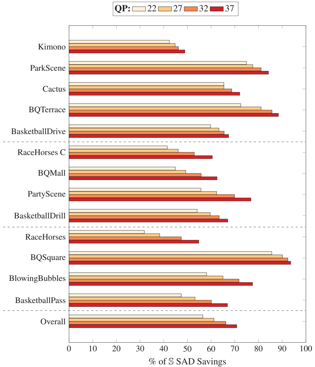
Figure 6.4 Percentage of square SAD operation savings, per sequence, for the proposed solution, when compared to HM-CBSEA.
