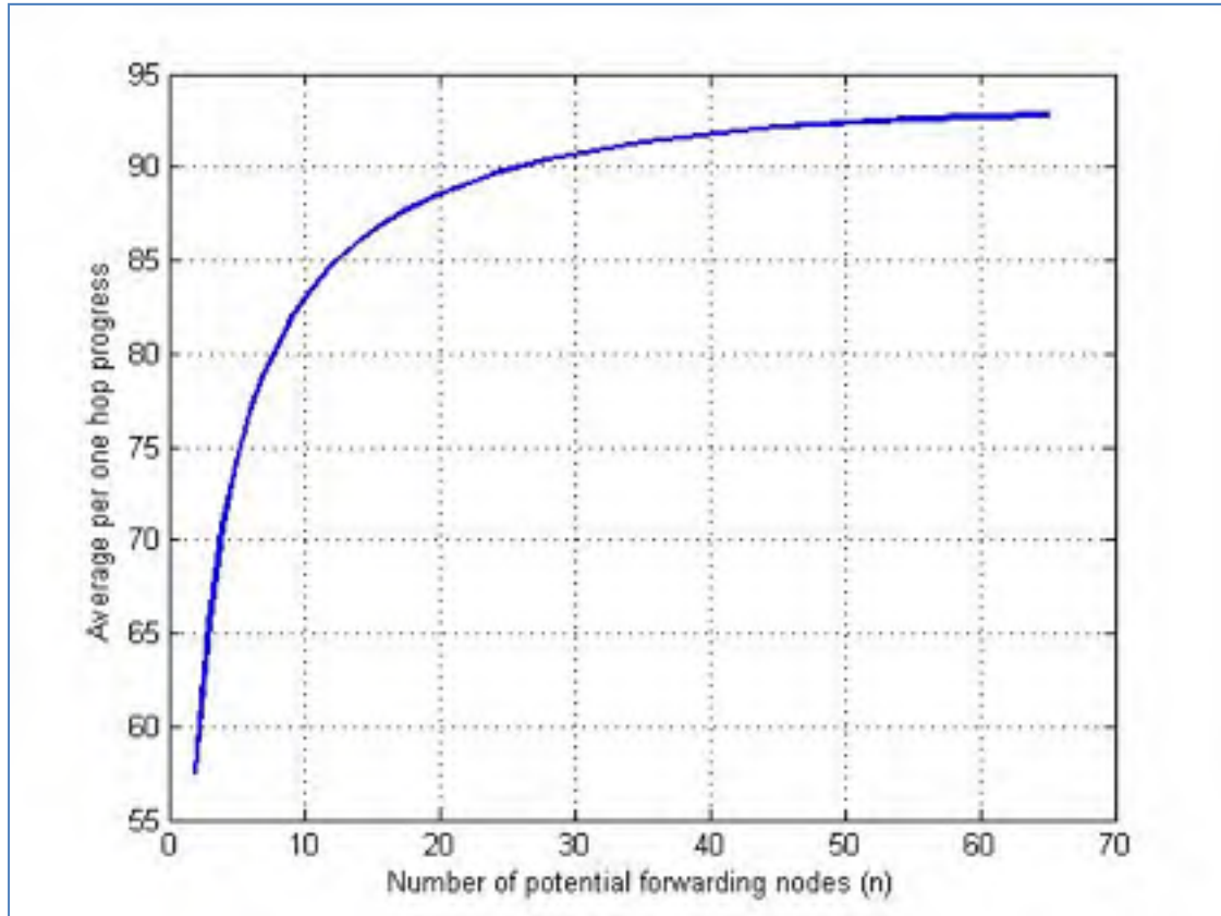
Figure 2.5 The relationship between the average value of Z ( \overline{Z_{def}} ) and the number of potential forwarding nodes ( n ) at R = 100m
