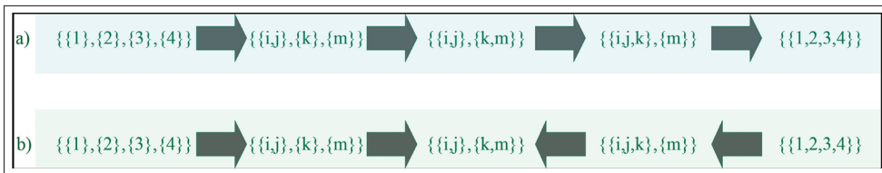
Figure 2.9 Feasible moves allowed by regulator for two weighting rules a) w_p = 0, w_u = 1 and b) 5w_p = w_u . Each of these diagrams shows the possible and allowed moves from any status quo coalition structure
