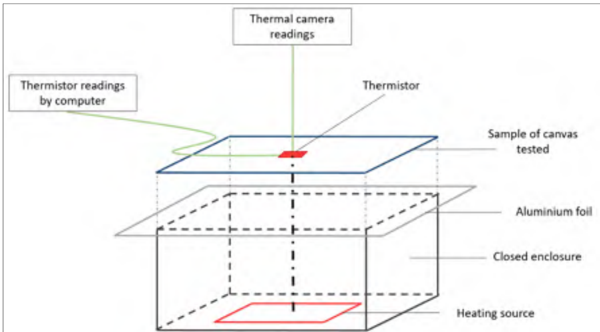
Figure 10 Experimental set-up diagram of emissivity measurements
