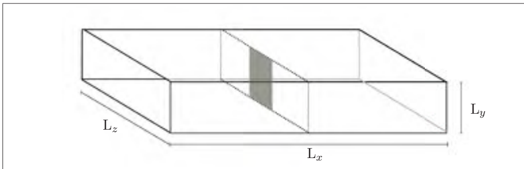
Figure 2.1 Infinite actuator strip validation setup. The shaded region corresponds to the surface.
