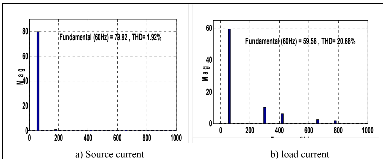
Figure 3.22 Harmonic spectrum
