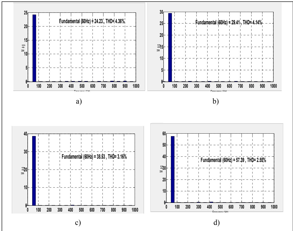
Figure 3.4 Source current harmonic spectrum at different V_{dref}
