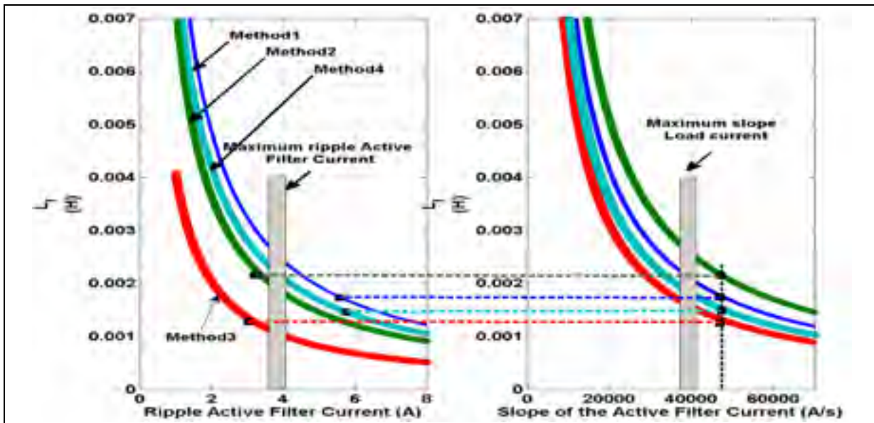
Figure 3.14 Comparison of different methods based on the minimum filter slope current
