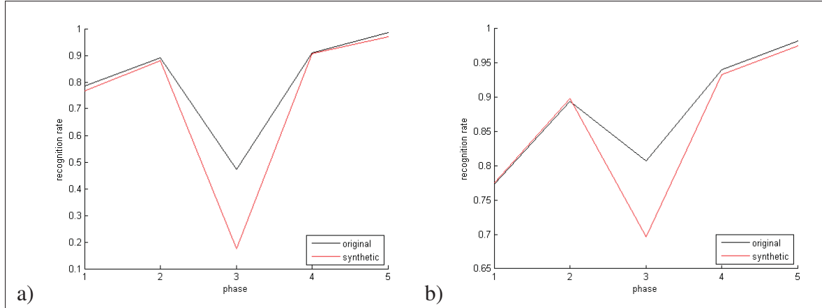
Figure 6.12 Recognition rate for the forgetting scenario a) without EML, b) with EML. Phase 1 learns and recognizes samples from all classes, Phase 2 learns and recognizes samples from all classes except one, phase 3 does not learn but recognizes the unused class from phase 2, and phase 4+ learn and recognize samples from all classes.
