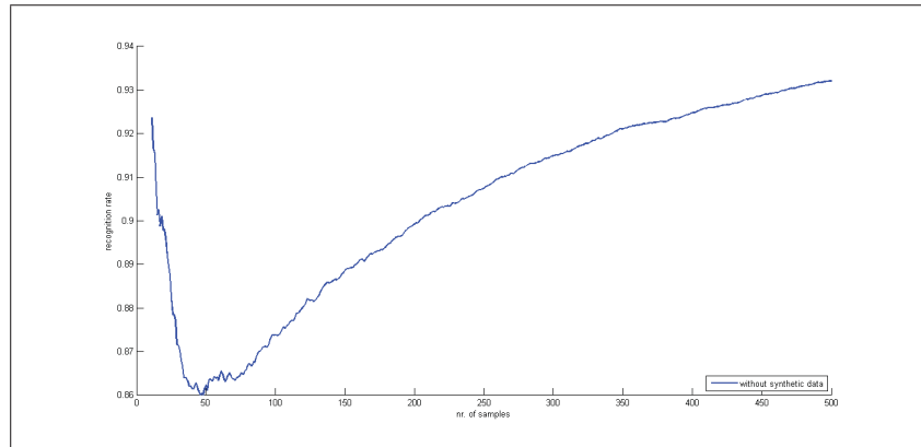
Figure 0.4 The problem of missing data. At the beginning of the learning/recognition process occurs the lack of data resulting into high variance visible by the drop in recognition rate in the figure.
