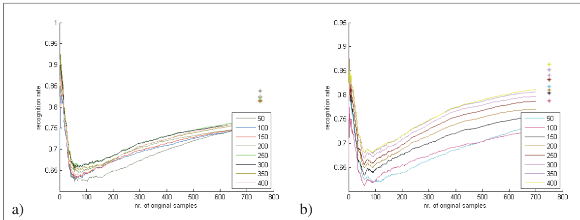
Figure 6.10 Comparison of different times to stop the generation of synthetic samples, i.e. different number of original samples for which synthetic samples are generated: a) without EML and b) with EML. At the very right an error on last 100 samples is visualized by stars to show the converged recognition rate of the system.
