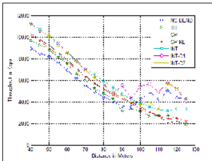
Figure A I-11 Network throughput for Diamond Topology vs. A-B distance
