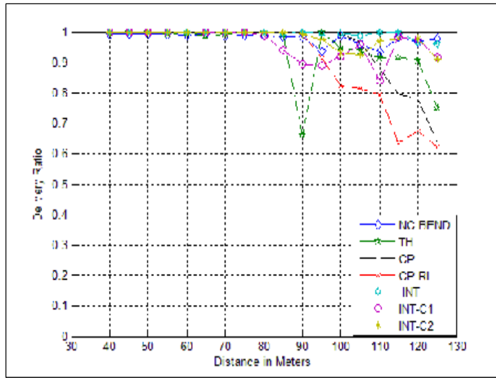
Figure A I-12 Delivery Ratio for Diamond Topology vs. A-B distance
