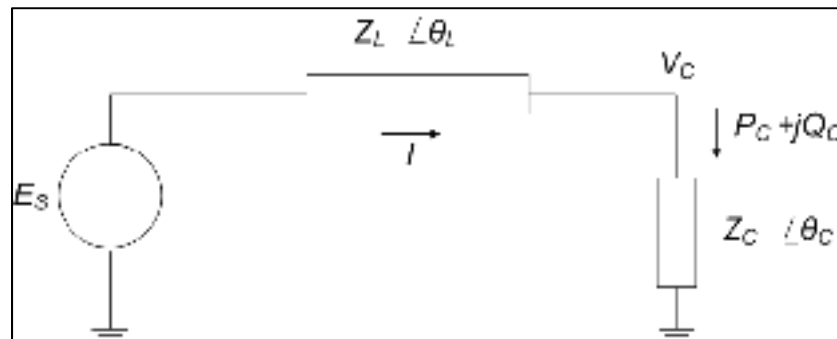
Figure 2.17 Circuit simple
