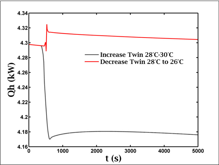
Figure 3.16 Impact of the water entry temperature on Q_h
