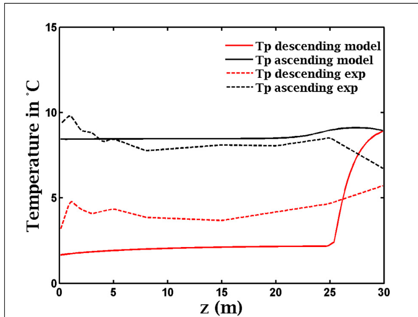
Figure 4.10 Profile of the temperature in the borehole after 150 seconds following the launch of the compressor
