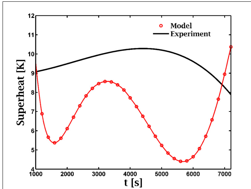
Figure 2.19 Superheat
