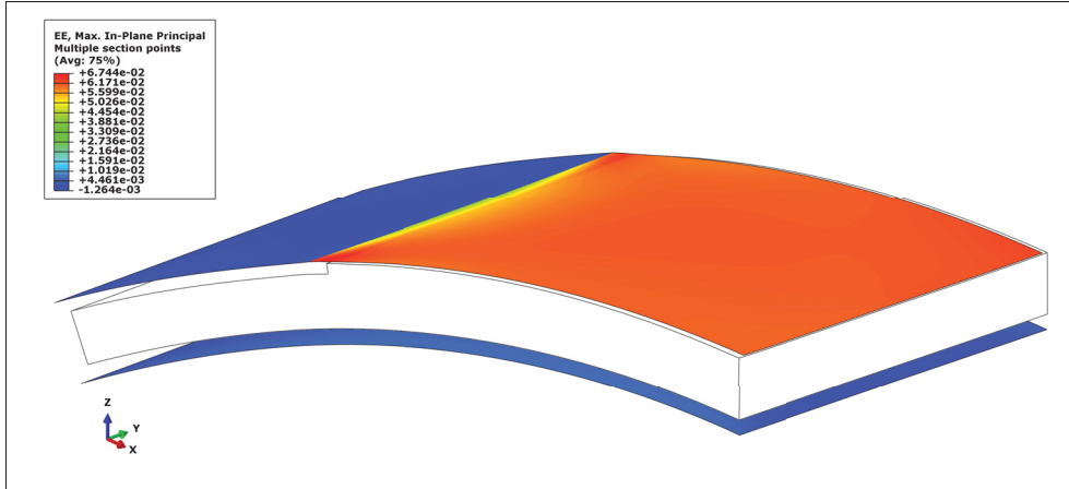
Figure 3.11 In-plane principal strains ( mm/mm ) on FEM model at 375 Nm
