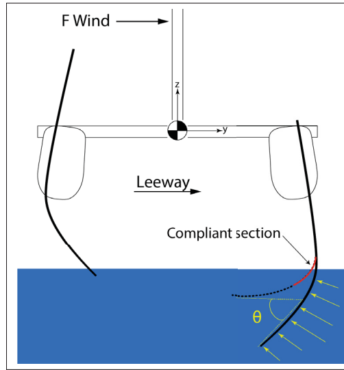
Figure 3.2 Deflected compliant foil with a 55° angle ( \theta )
