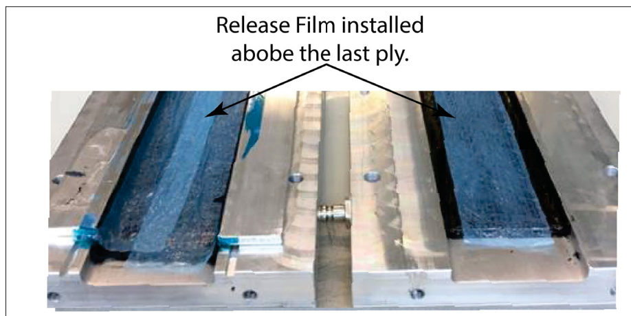
Figure 3.22 Release film installed above the last ply
