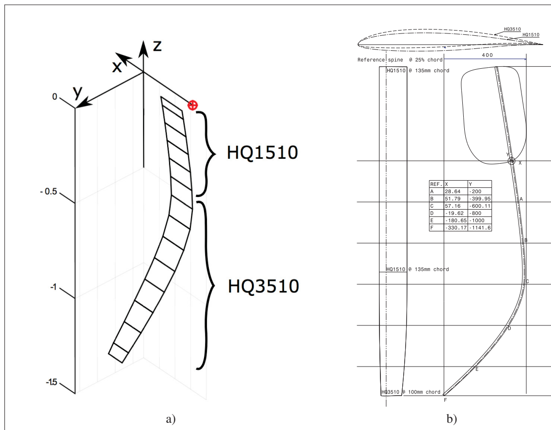
Figure 2.4 EH1 Hydrofoil Drawing Designed by C. Dransfeld
