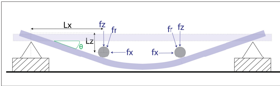
Figure 3.30 Forces and levers diagram on FPB Test
