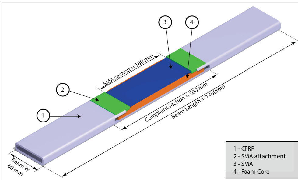
Figure 2.12 Compliant section prototype CAD
