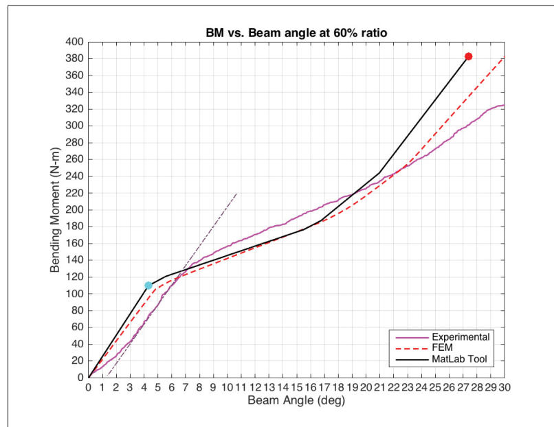
Figure 3.33 Tangent curve on first slope exp. data
