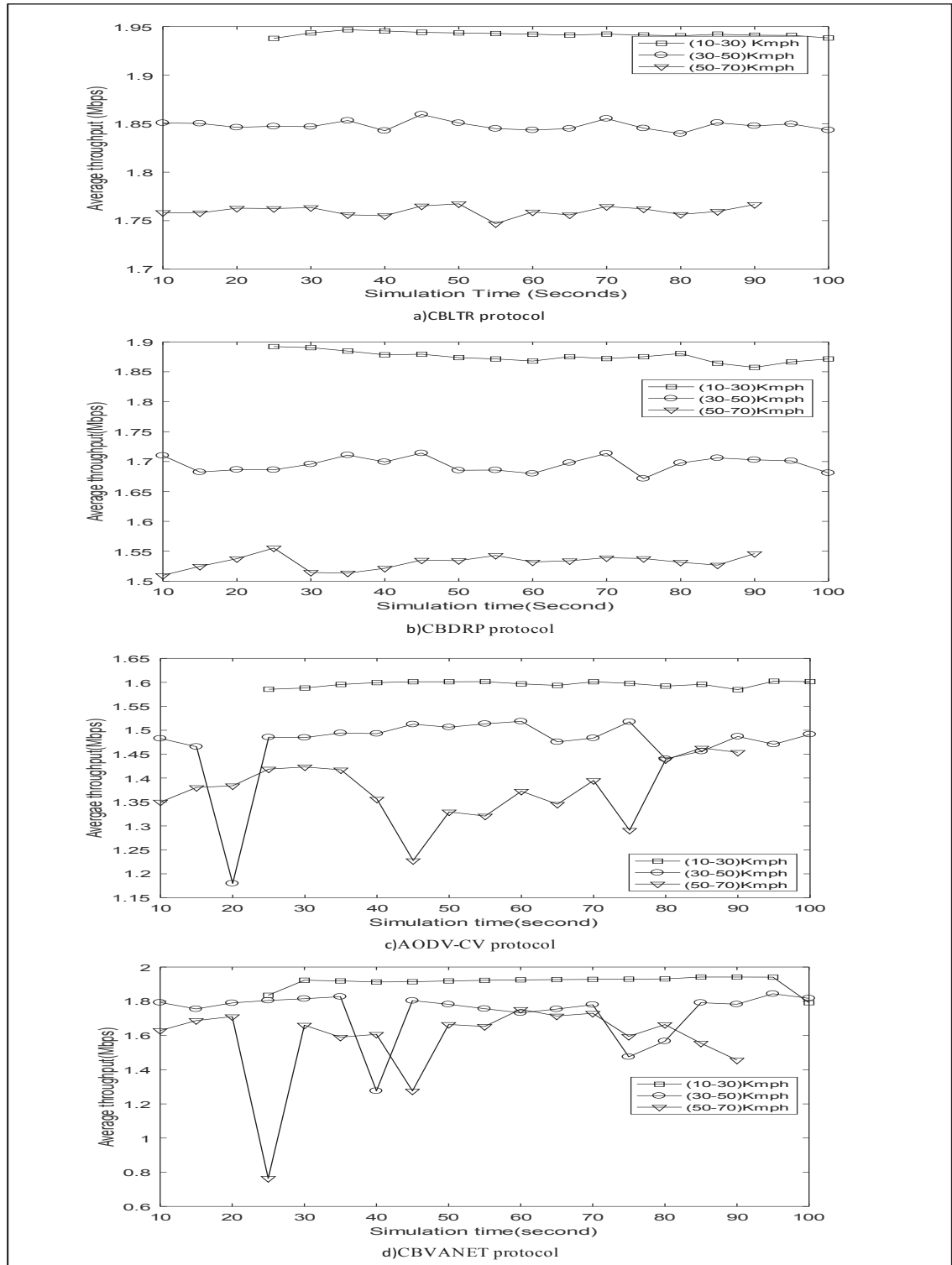
Figure 1.14 Average throughput calculation for bidirectional segment, Figure (a) represents our proposed protocol CBLTR protocol, Figure (b) represents CDBRP protocol, Figure (c) represents AODV-CV protocol, Figure (d) represents CBVANET protocol
