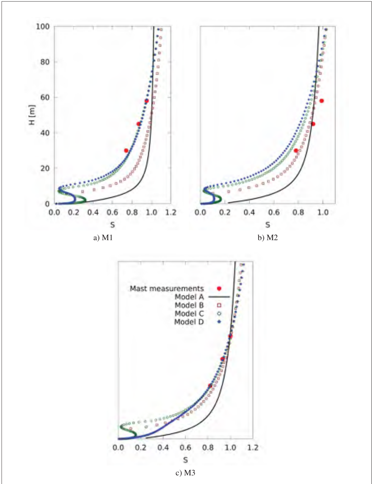
Figure 4.8 Results of the four model cases compared with mast mean results in terms of speed-up factor S = U/U_{ref,M3-top}
