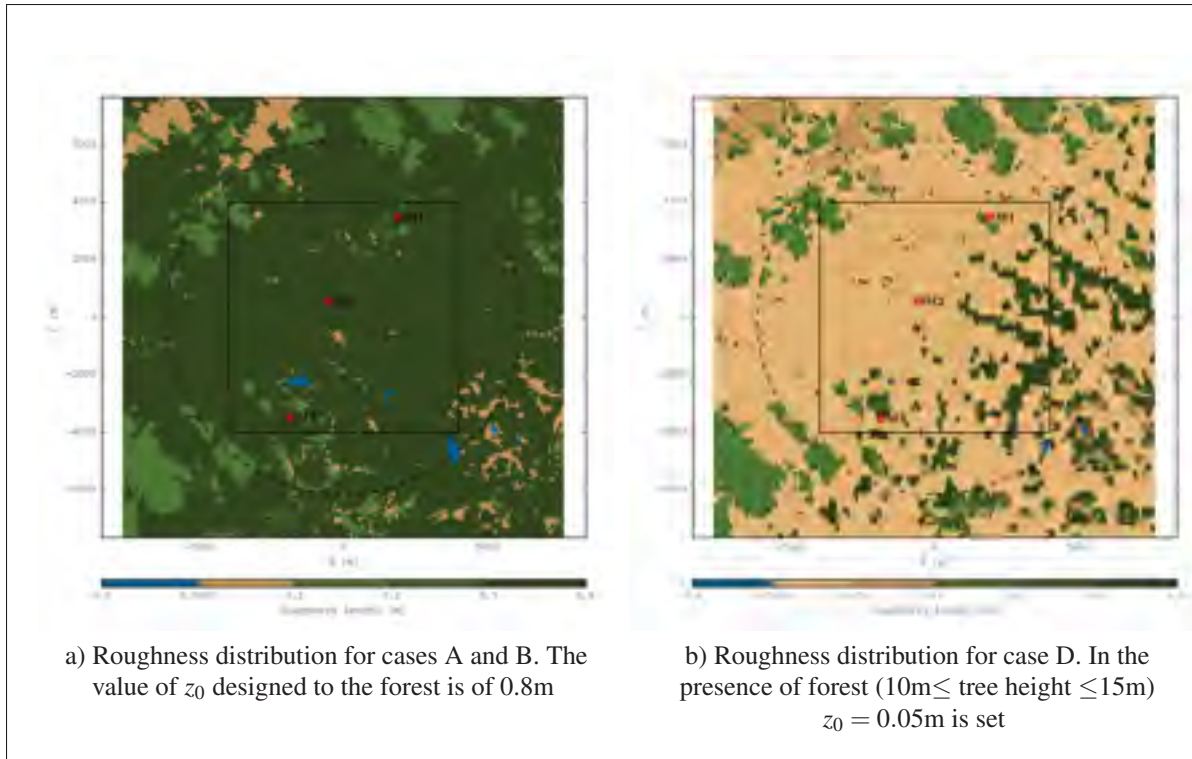
Figure 4.4 Roughness distribution
