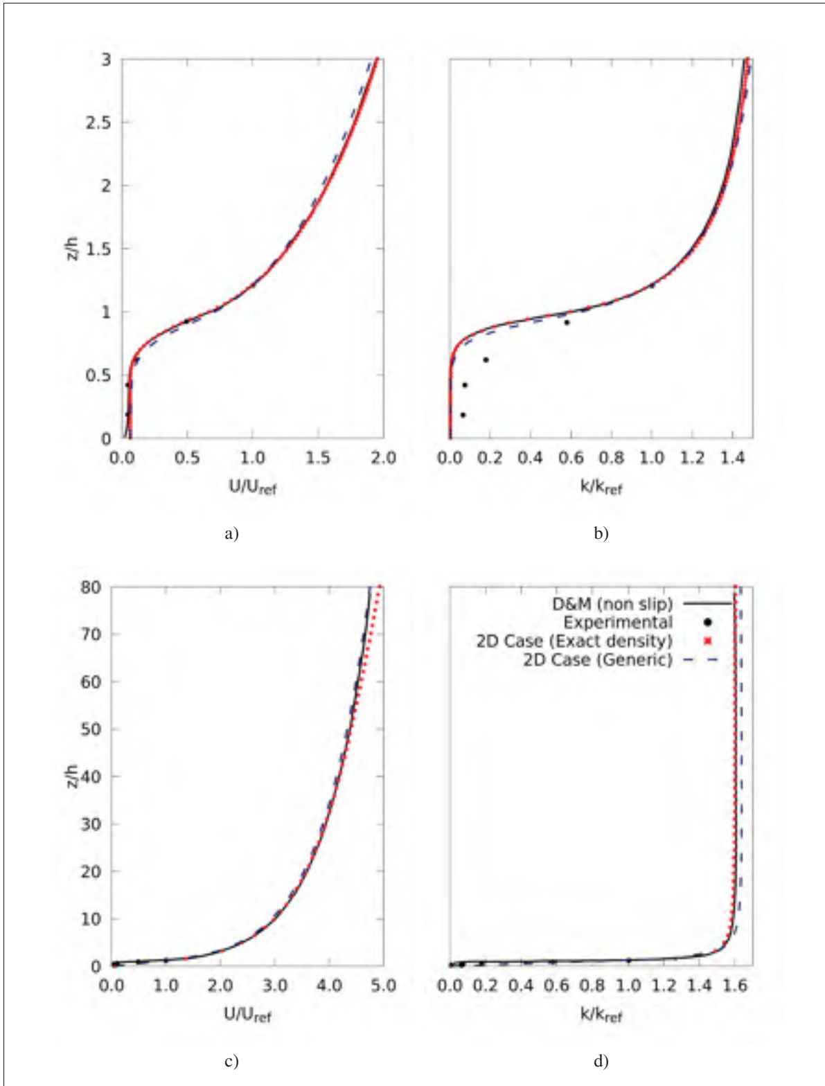
Figure 3.2 U and k distributions for 2D case with cyclic boundary conditions up to 30 and 800 m. Values are normalized at z/h=1.21
