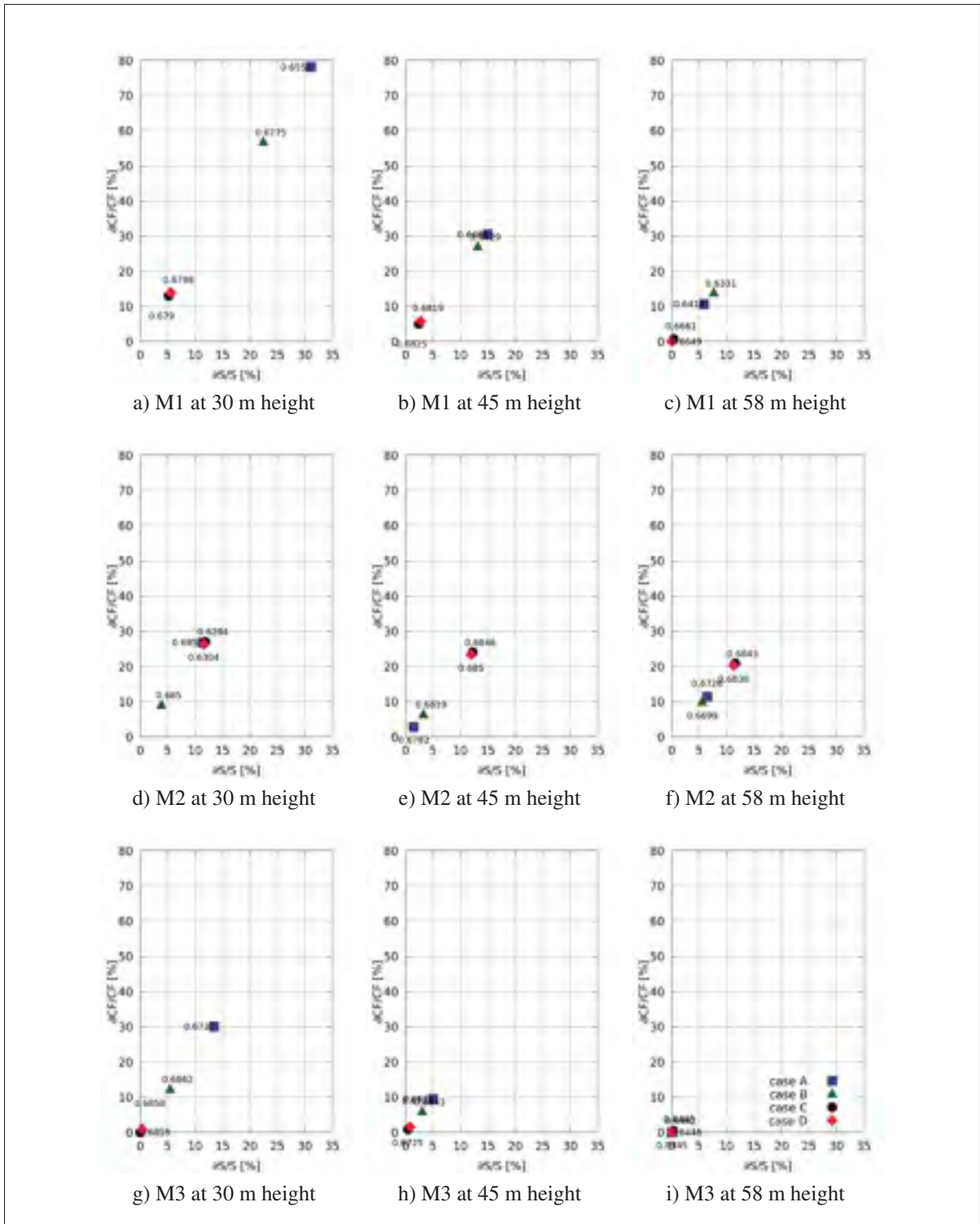
Figure 4.11 Percent error in capacity factor \frac{\partial CF}{CF} for 1% error in speed-up factor \frac{\Delta S}{S} for the four model cases. The labels show the values of the the absolute error in CF for an absolute error in S ( \frac{\partial CF}{\partial S} )
