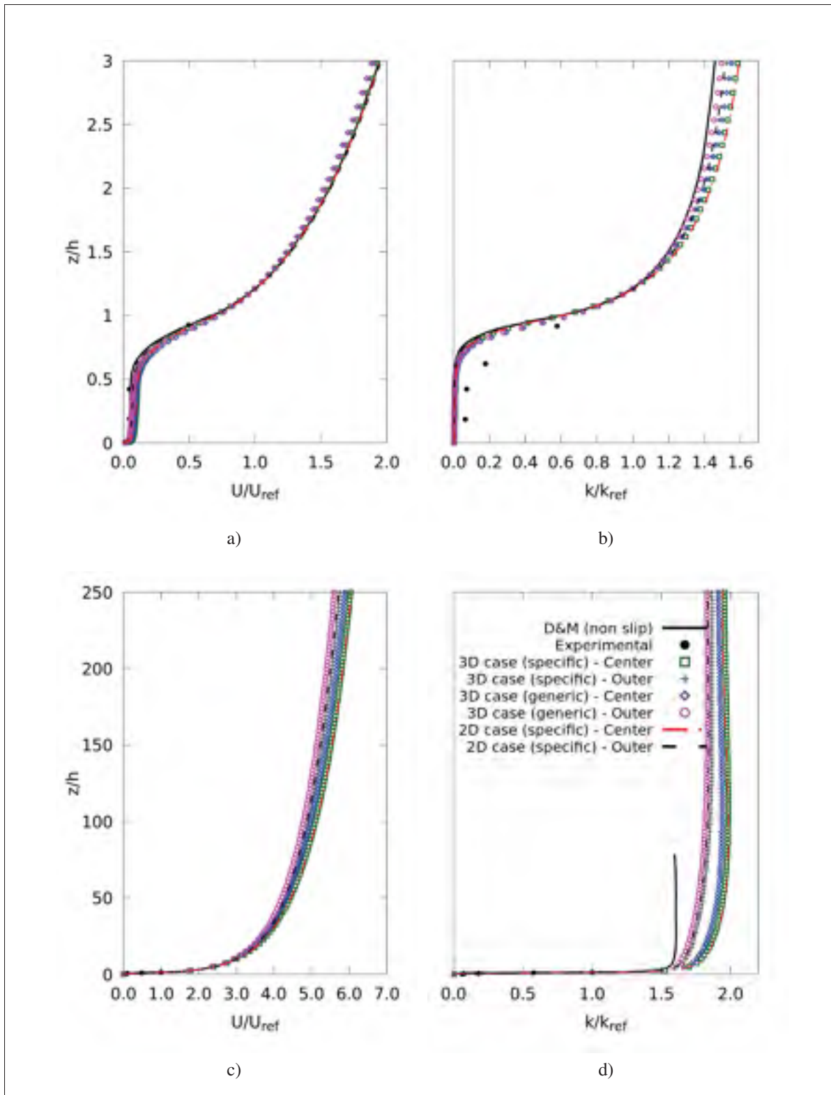
Figure 3.11 U and k distributions for 3D flat terrain case up to 30 and 2 500 m. Values are normalized at z/h=1.21
