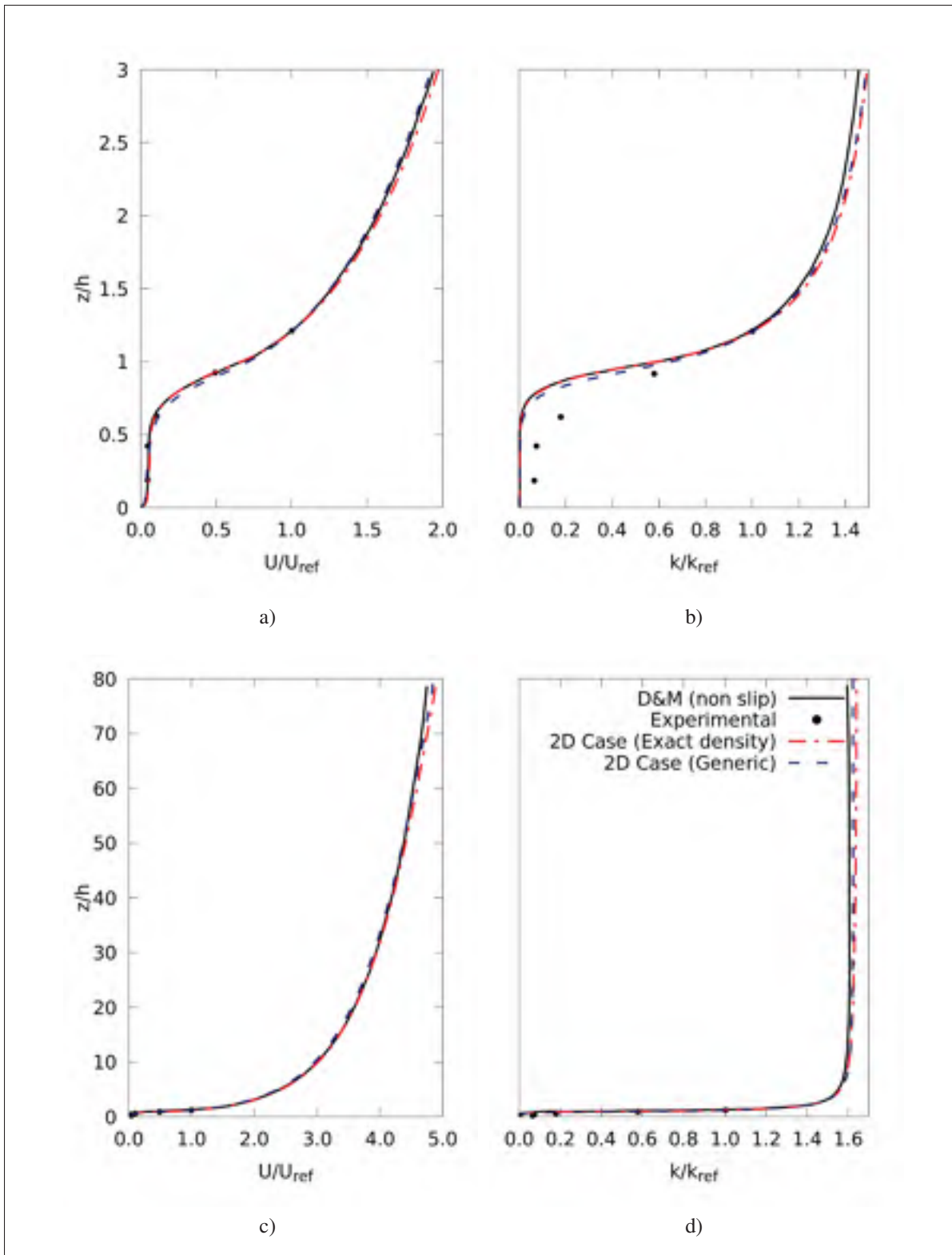
Figure 3.8 U and k distributions for 2D case with inlet-outlet boundary conditions up to 30 and 800 m. Values are normalized at z/h=1.21
