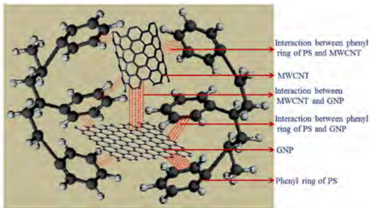
Figure 1.3 - Schematic representation for \pi - \pi interactions between GnP, MWCNT, and PS in hybrid nanocomposites of PS/MWCNT/GnP (Maiti et al., 2013)
