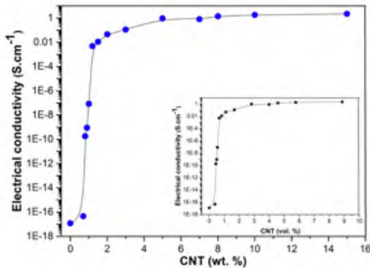
Figure 2.3 - Electrical conductivity of SEBS/CNT nanocomposites at different CNT weight and volume fractions
