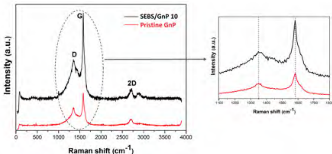
Figure 3.7 - Raman spectra of pristine GnP and SEBS/GnP nanocomposites with 10 wt.% GnP (on the left), and blow-up of the spectra in the 1100-1800 \text{cm}^{-1} region (on the right)
