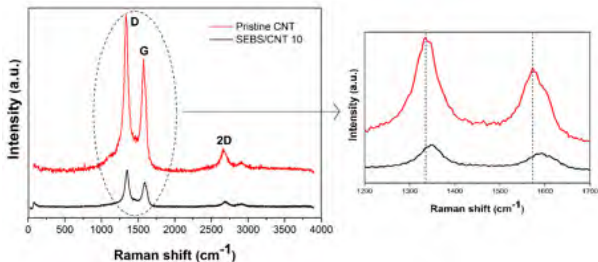
Figure 2.1 - Raman spectra of pristine CNT and SEBS/CNT nanocomposite with 10 wt. % of CNT and blow up of the spectra in the 1200-1700 \text{cm}^{-1} region
