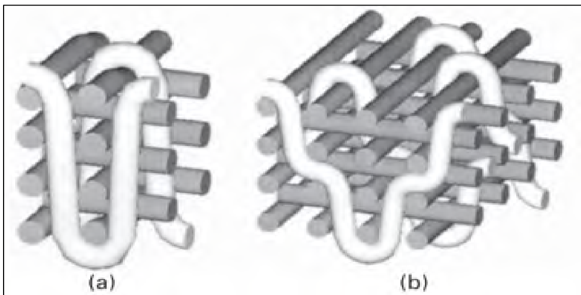
Figure 1.8 Exemples de tissage 3D multicouches a) orthogonal b) interlock (De Luycker, 2009)
