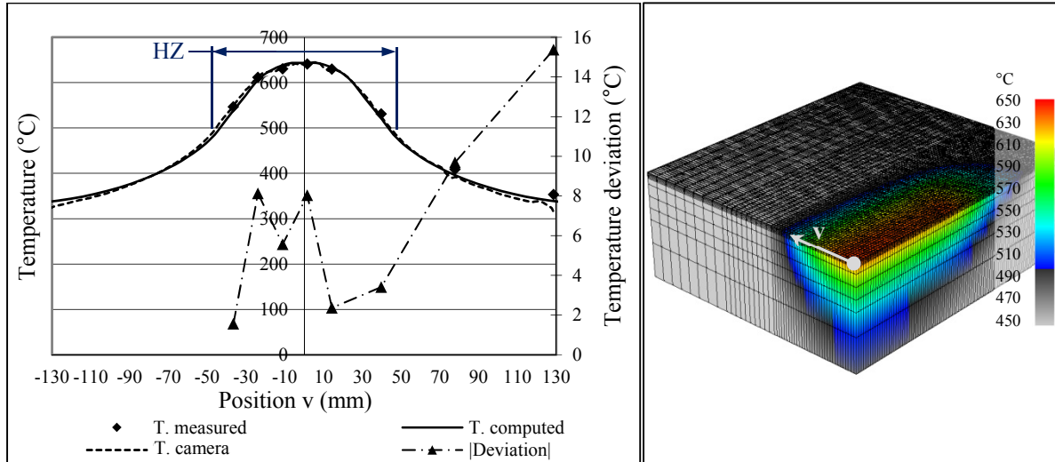
Figure 3.13 Comparison between computed and measured lateral temperature profile ( W = 35 mm)
