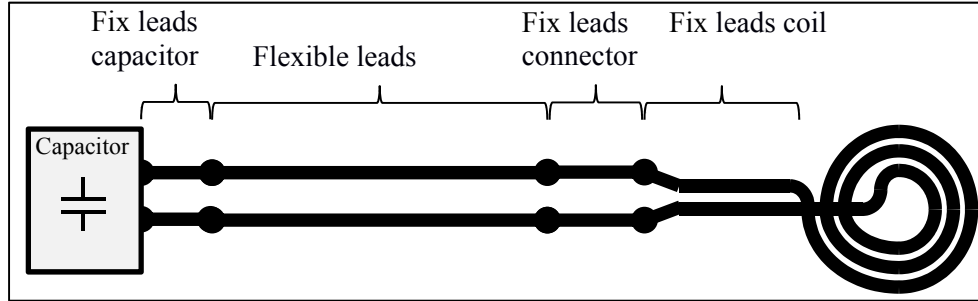
Figure 5.4 Simplified representation of the RLC circuit leads
