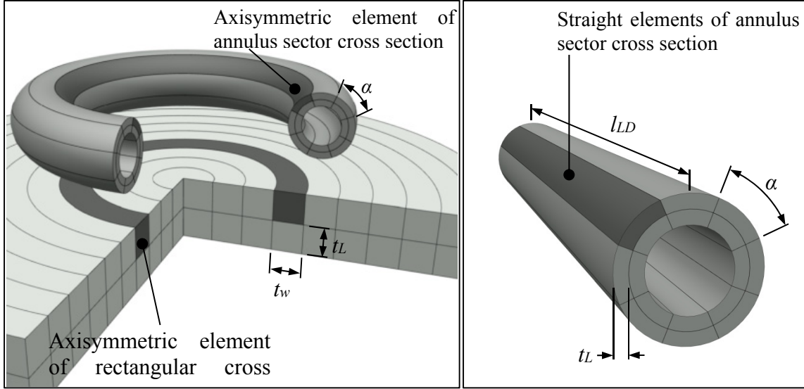
Figure 5.5 Examples of discretization of a round conductor above a conductive medium into axisymmetric elements (left) and discretization of a straight round conductor into straight elements (right) ( N_c = 16 , N_w = 20 , N_L = 2 , N_t = 1 )
