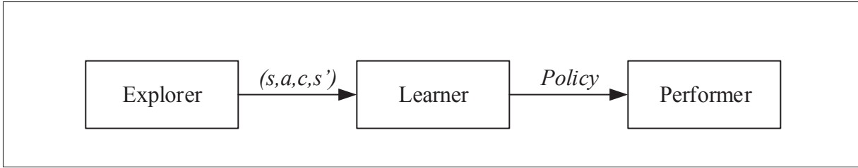
Figure 5.9 Three agents of a batch-mode reinforcement learning system.
