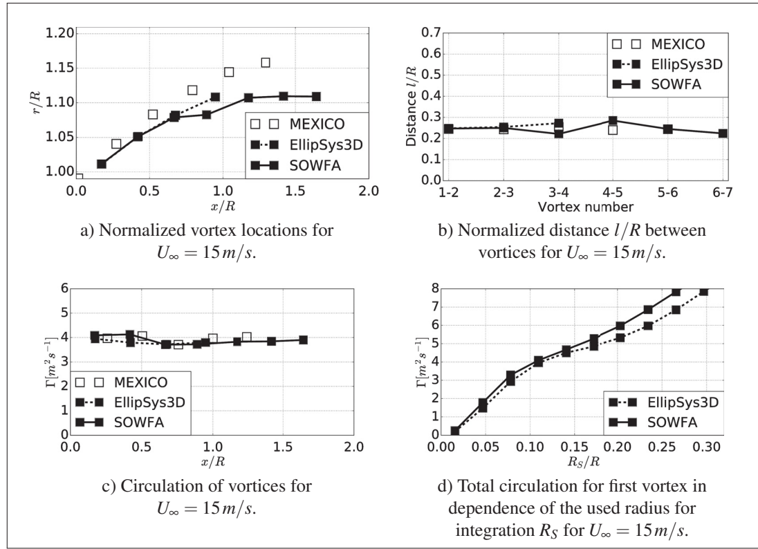
Figure 4.8 Comparison of the vortex properties in the near wake.
