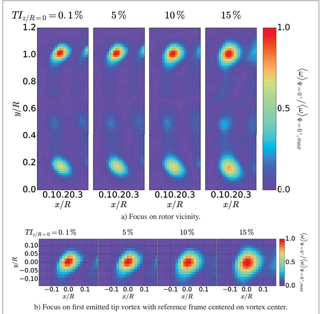
Figure 6.9 Phase-averaged normalized vorticity \langle \omega \rangle_{\Psi=0^\circ} / \langle \omega \rangle_{\Psi=0^\circ, max} in sheared flow for different longitudinal turbulence intensities TI_x at hub position.
