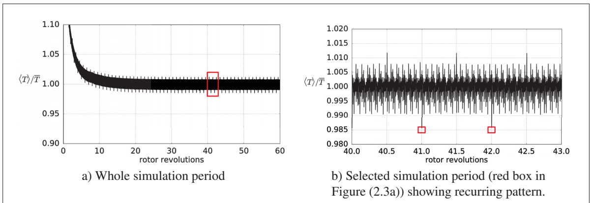
Figure 2.3 Variation of normalized rotor torque \langle T \rangle / T_{ref} over rotor revolution. The mean \langle T \rangle is obtained via the lift forces acting on the rotor blades.
