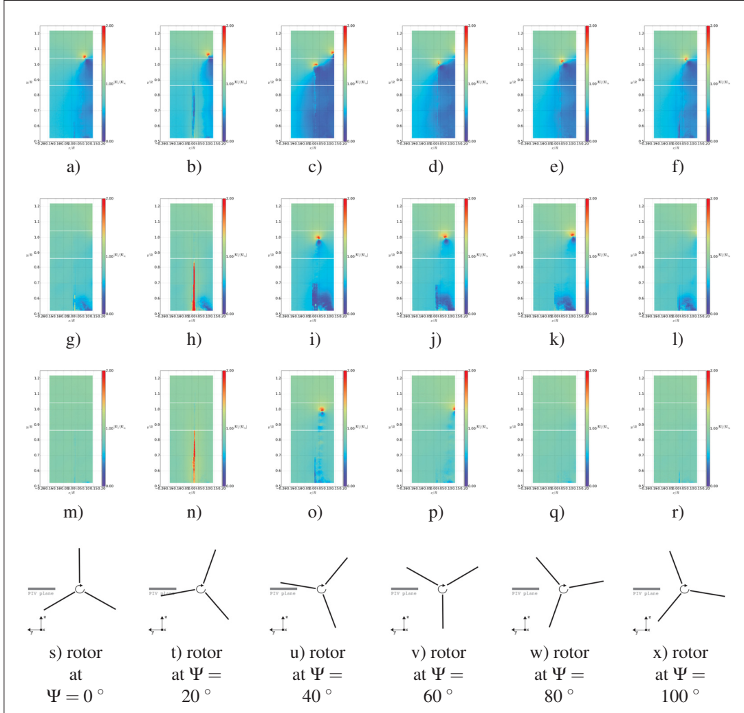
Figure 3.7 Phase-averaged velocity magnitudes |\mathbf{U}|/U_\infty for U_\infty = 10\text{ m/s} (first-row), U_\infty = 15\text{ m/s} (second-row), U_\infty = 24\text{ m/s} (third-row) for different rotor positions \Psi (last-row).
