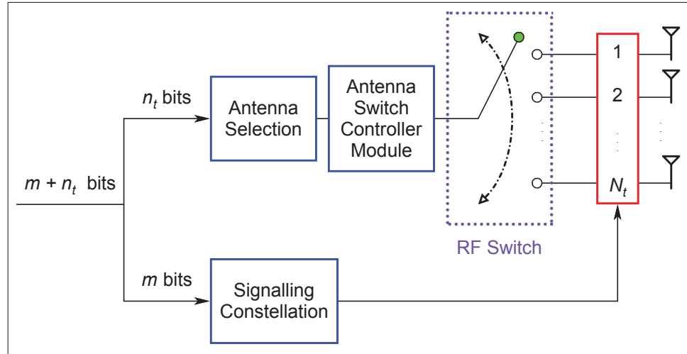
Figure 1.1 Block diagram of the SM transmitter
