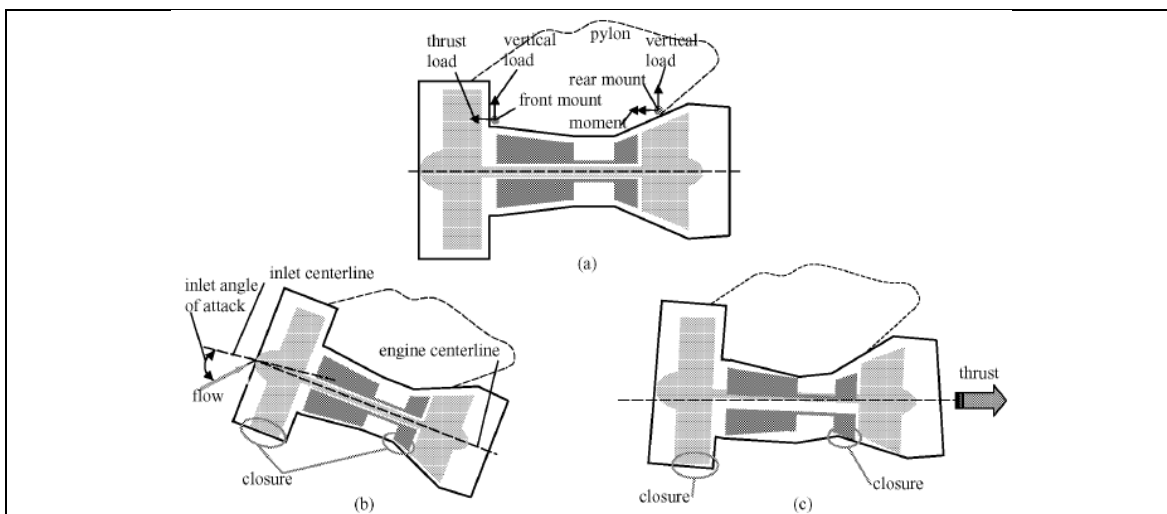
Figure 6.4: (a) Engine mounts and load paths, (b) Closures due to aero loads, (c) Closures due to thrust loads
