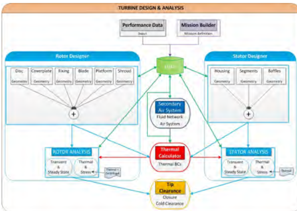
Figure 4.3: Tip clearance calculation methodology
