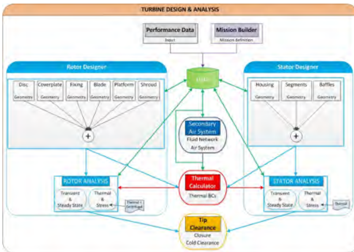
Figure 3.1 : Tip clearance calculation methodology
