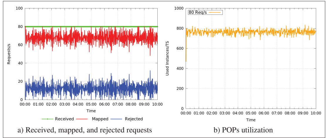
Figure 4.8 80 Requests/s
