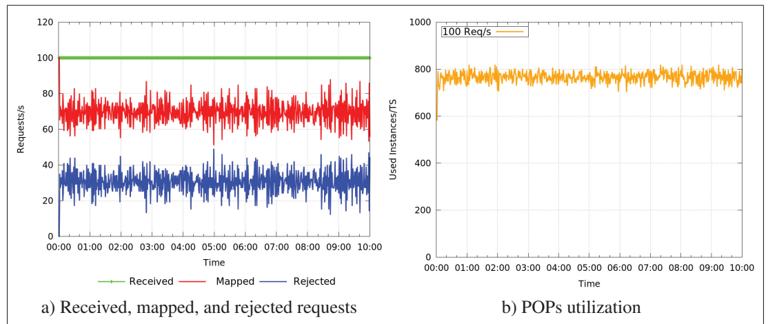
Figure 4.9 100 Requests/s
