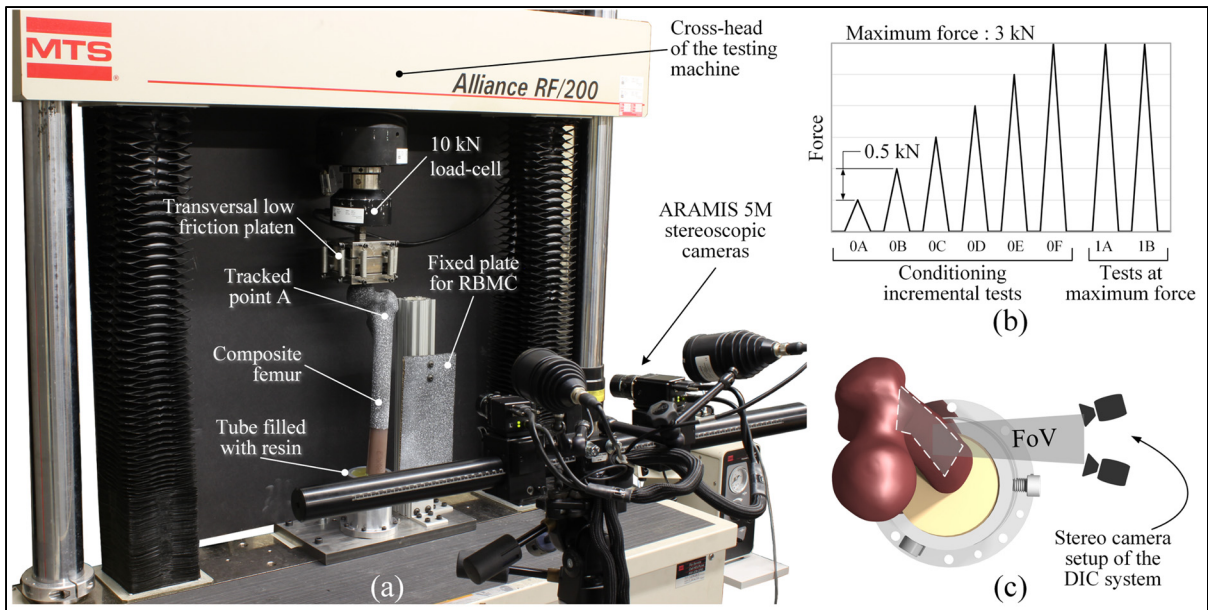
Figure 3.3 (a) Experimental devices and the testing setup, (b) load protocol followed for each femur, (c) top view showing the schematic coverage of the FoV
