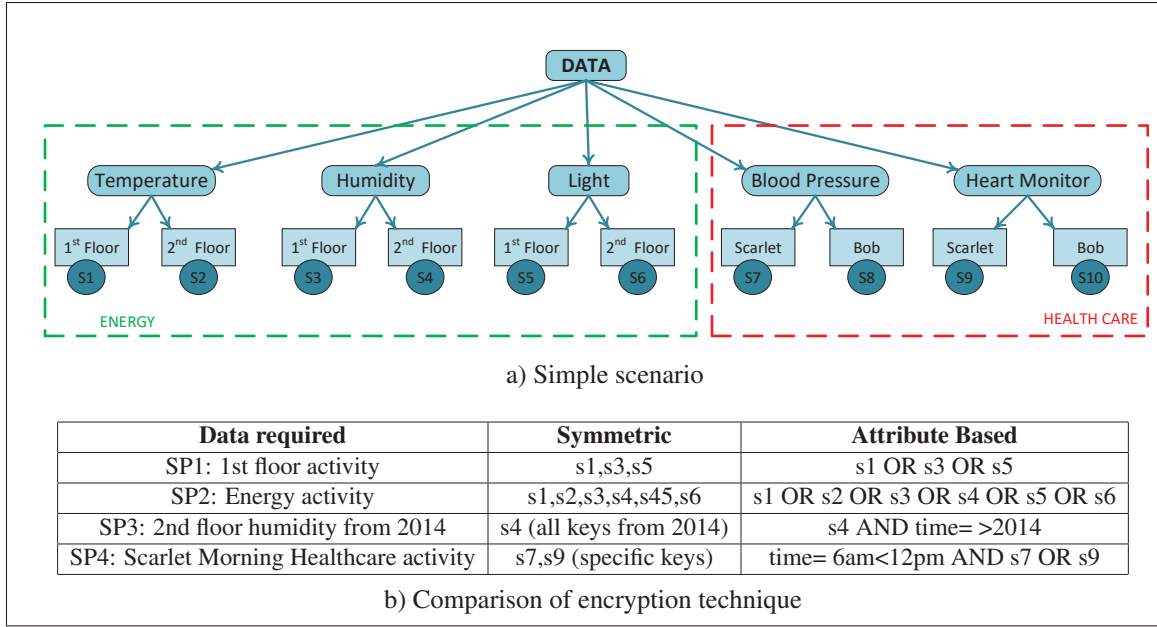
Figure 1.7 ABE representation
