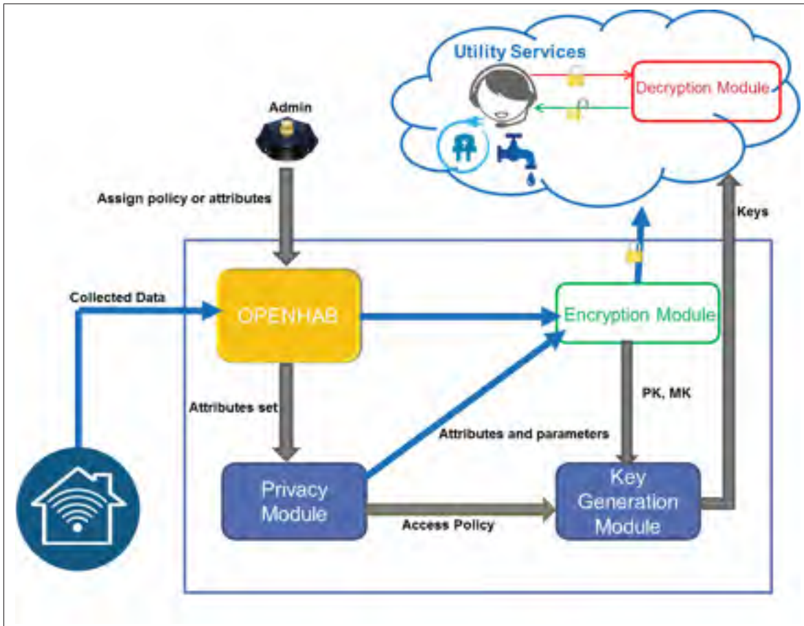
Figure 3.1 Architecture Overview.
