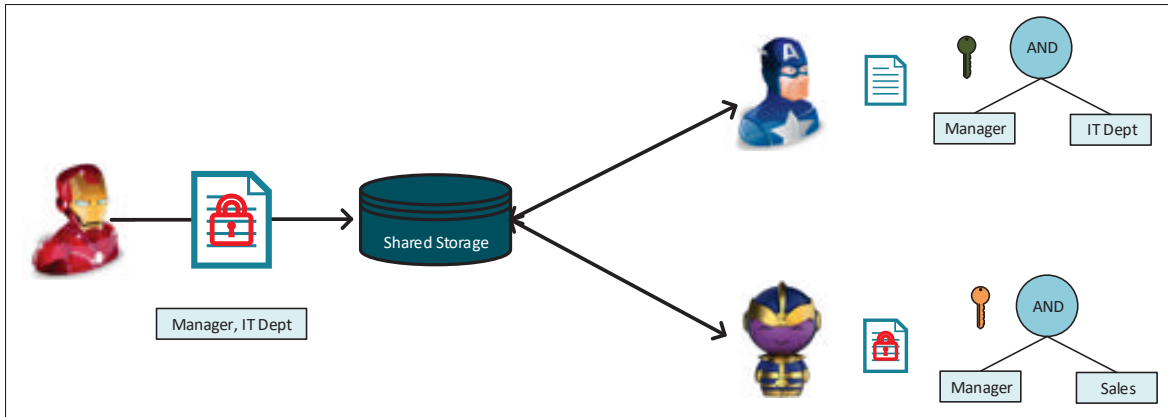
Figure 1.9 KP-ABE
