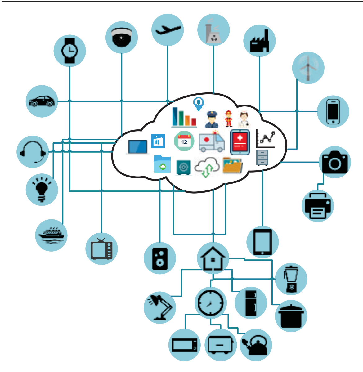
Figure 0.1 IoT Overview.
