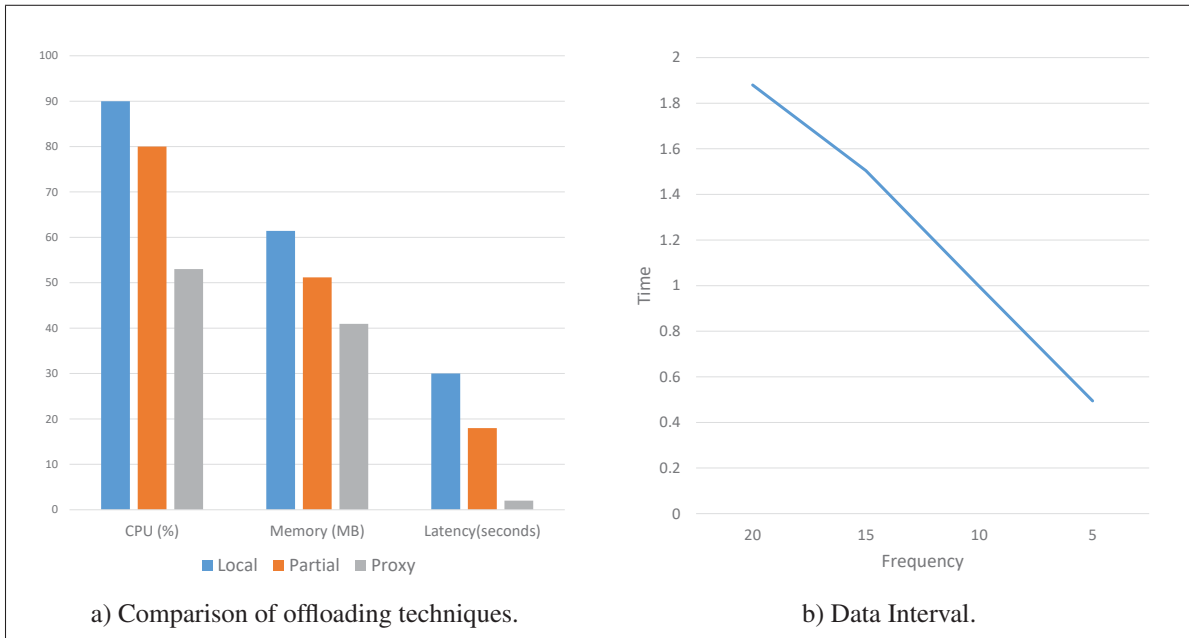
Figure 4.5 Experimentation on different techniques and settings.
