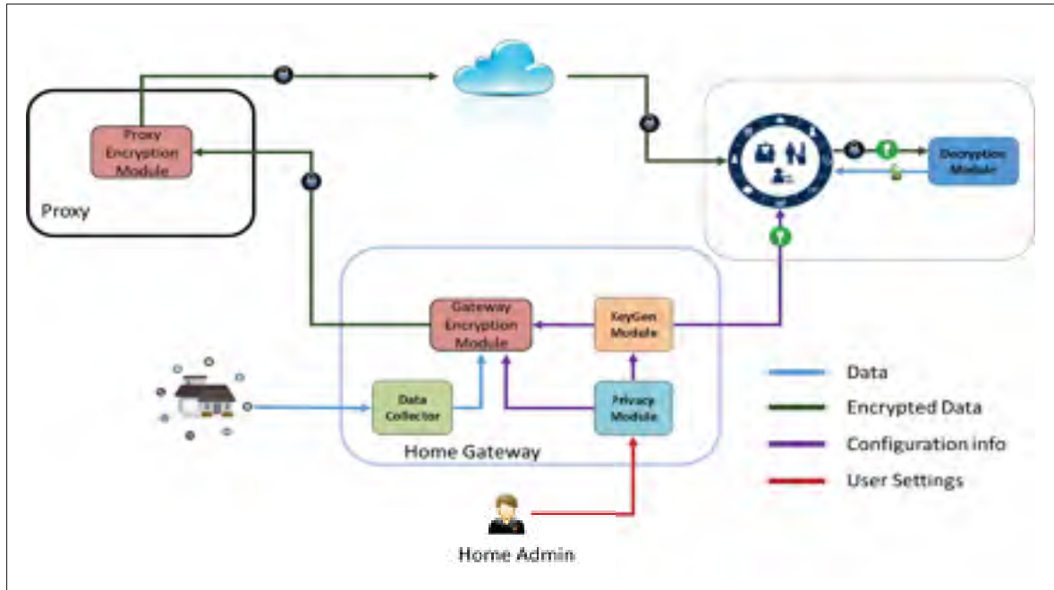
Figure 4.2 Outsourcing Architecture Overview.
