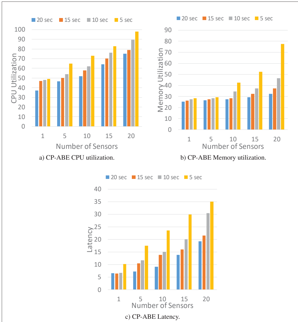
Figure 3.9 CP-ABE results.
