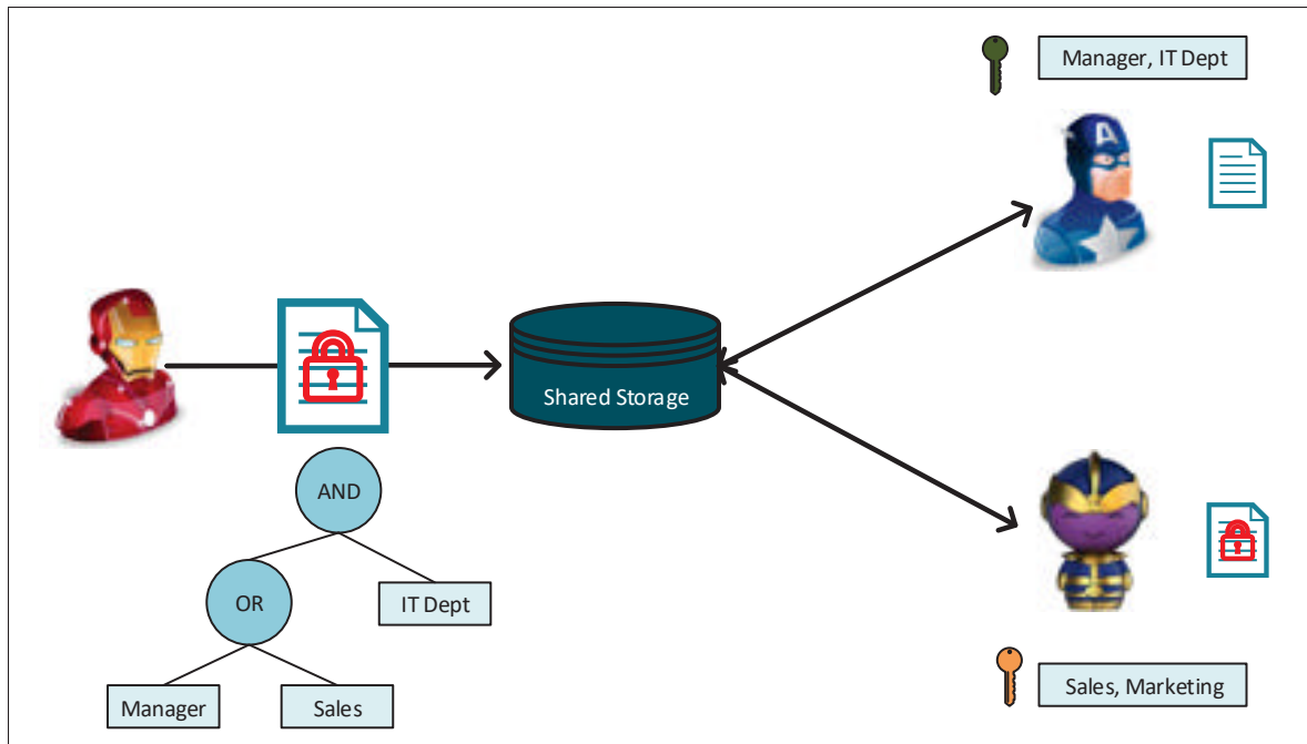
Figure 1.8 CP-ABE
