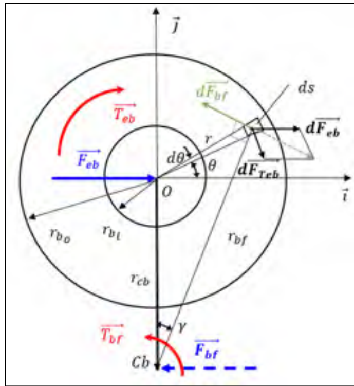
Figure 3.2 Free body diagram under head
