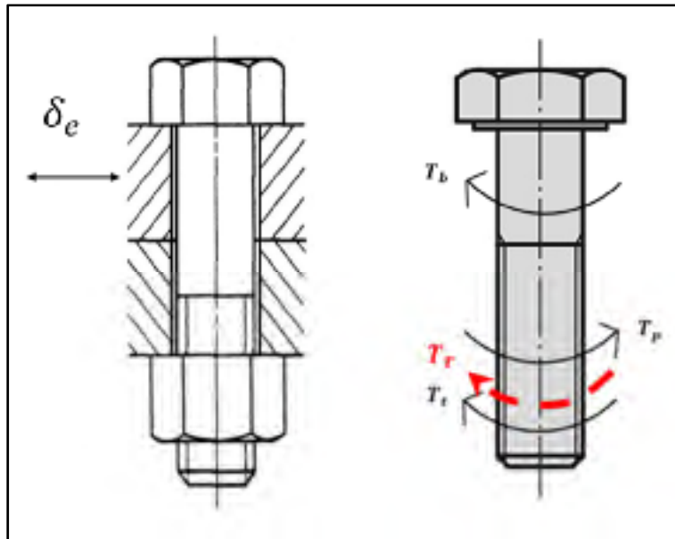
Figure 3.1 The bolted joint assembly under a lateral movement and torques T_b , T_t , T_p and T_r
