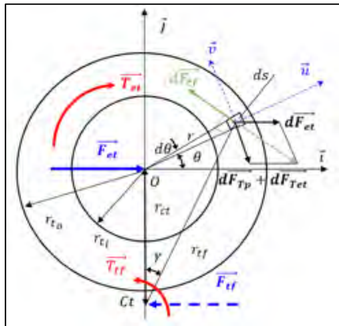
Figure 3.3 Free body diagram in the threads
