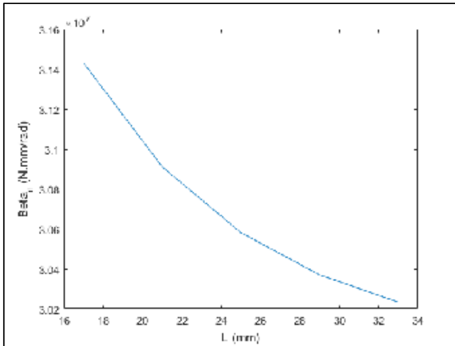
Figure 3.8 Bending stiffness \beta_N versus the grip length L
