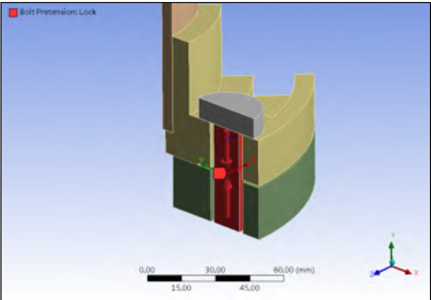
Figure 2. 17 Bolt Pretension
