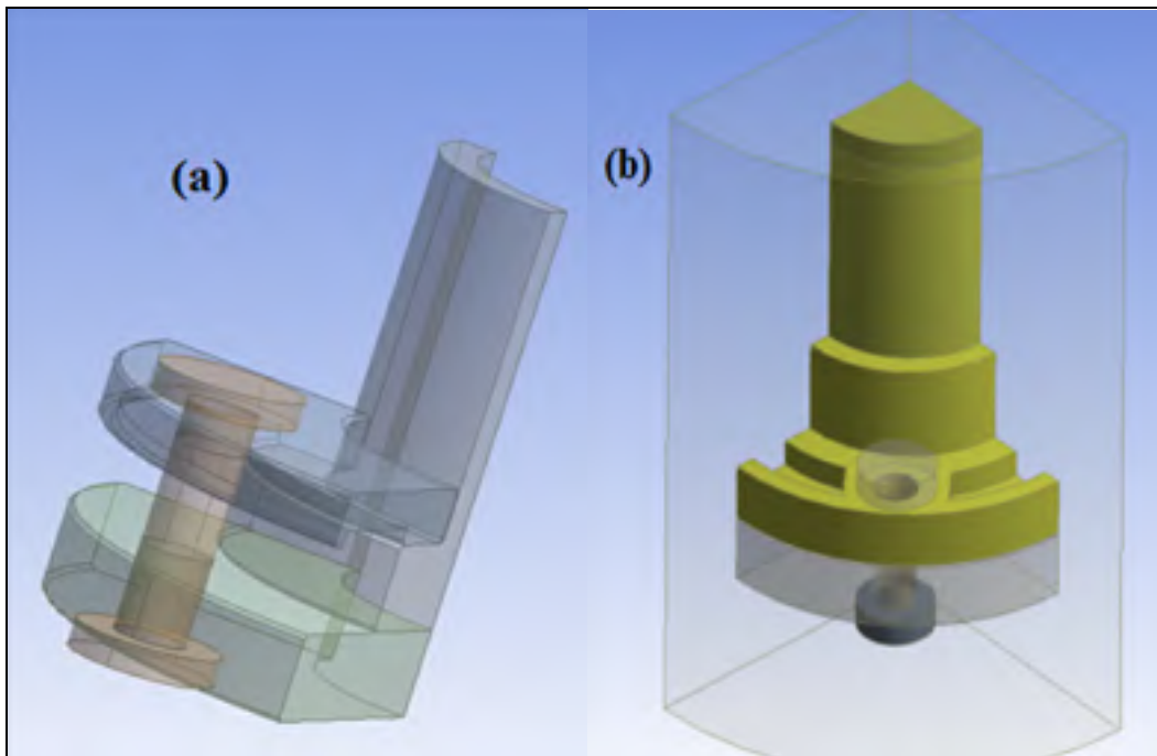
Figure 2. 15 (a) HDPE modeling in CATIA, (b) PVC model in ANSYS.
