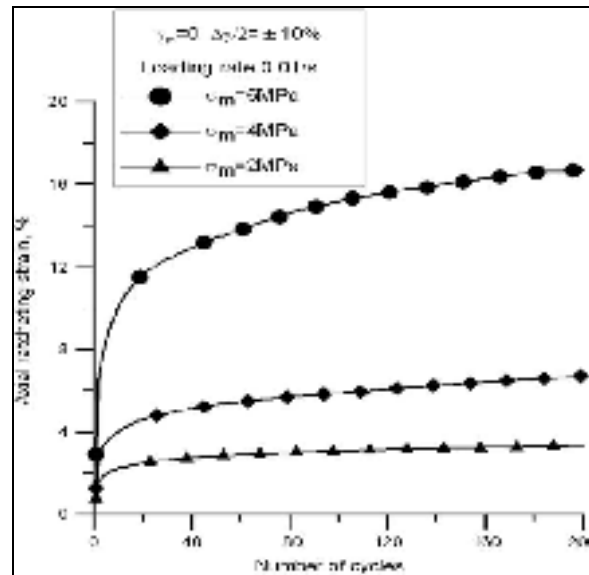
Figure 1. 27 Effect of constant axial load (Zhang and Chen, 2009)
