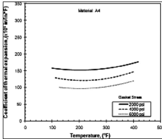
Figure 1. 29 Influence of applied load on the CTE (Bouزيد and Benabdullah, 2015)
