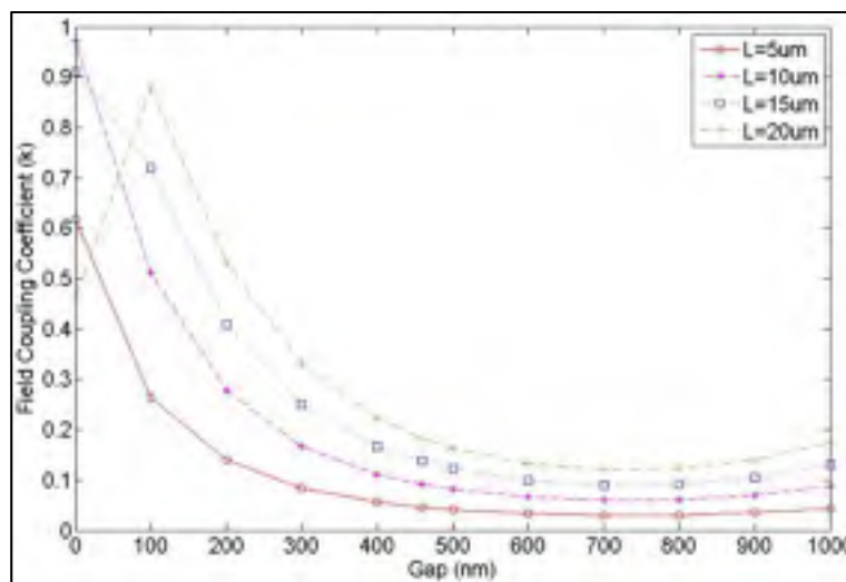
Figure 4.5 Field coupling coefficient ' \kappa ' vs gap, \lambda=1550 nm, coupler length L=5 \mu\text{m} , L=10 \mu\text{m} , L=15 \mu\text{m} and L=20 \mu\text{m} , 400 nm x 400 nm waveguide, calculated using the waveguide mode solver with a 10 nm mesh size
