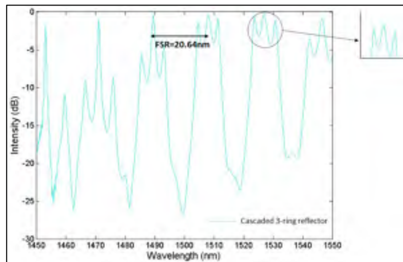
Figure 3.13 The reflection response of a serially coupled 3-ring reflector in a 2.5D-FDTD showing resonance peak splitting
