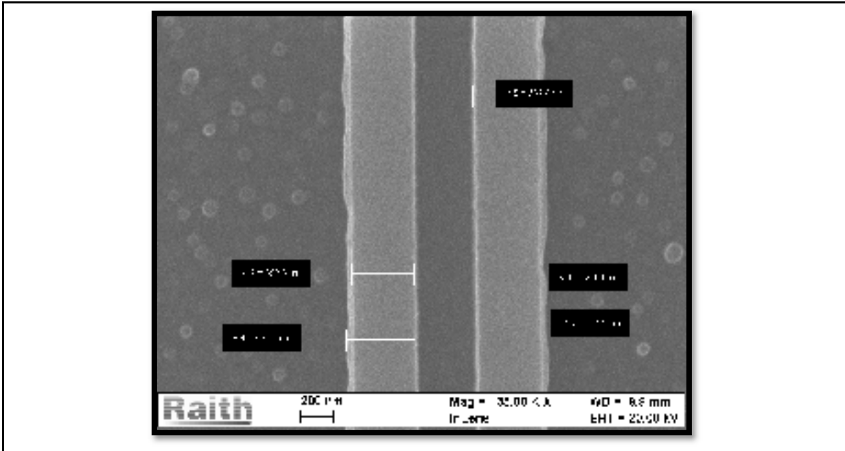
Figure 4.22 SEM image of a directional coupler of a fabricated large RR
