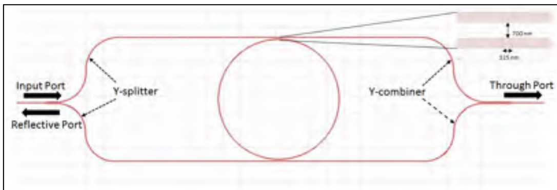
Figure 3.8 General schematic of a single ring reflector based on \text{Si}_3\text{N}_4 waveguide with dimensions 435\ \text{nm} \times 435\ \text{nm}
