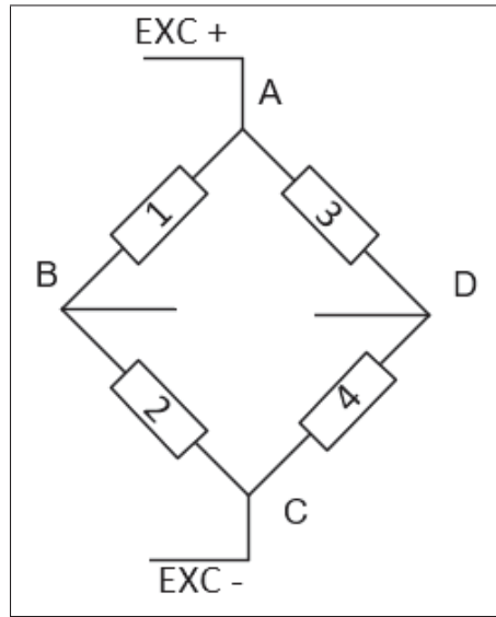
Figure 4.2 Pont de Wheatstone
