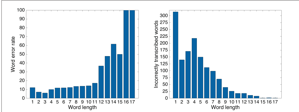
Figure 3.4 The word error rates and number of incorrect word recognitions corresponding to different lengths of words in the IAM database.
