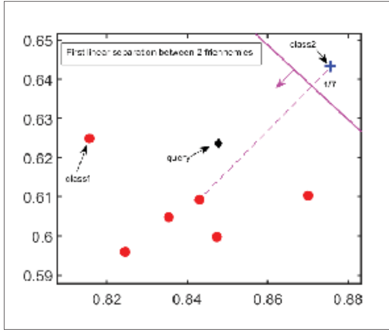
Figure 2.6 The frienemies separation proposed that is closer to the minority class (blue cross) with the pink classifier for a \lambda = \frac{1}{7} .
