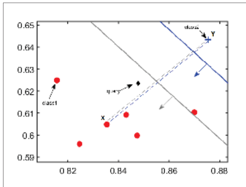
Figure 2.7 The difference between the frienemies separation in the midpoint (in gray) and the proposed separation (blue cross)
