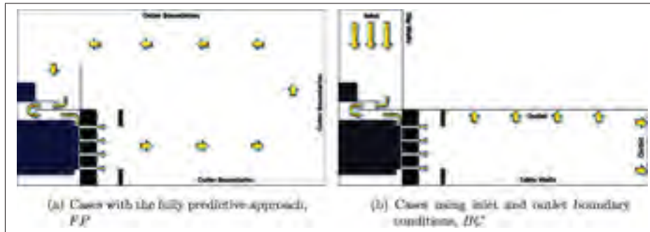
Figure 2.4 Geometry of generator used in Moradnia et al. (2014a).
