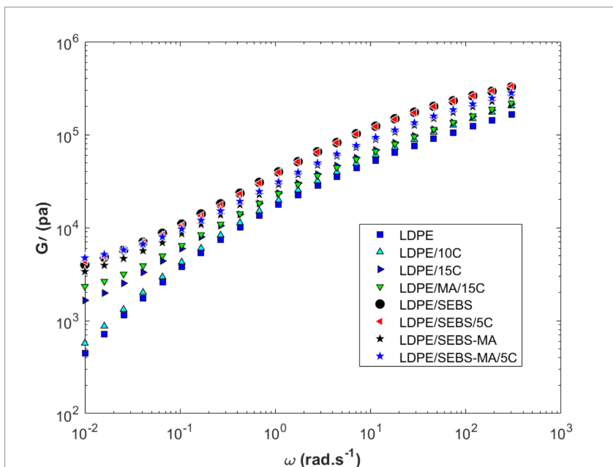
Figure 3-6 SAOS measurements of LDPE, SEBS blends and Clay-reinforced nanocomposites: Storage modulus ( G' ) as function of angular frequency ( \omega )
