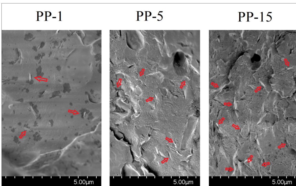
Figure 6-2 Scanning electron microscopy micrographs of PP-clay nanocomposites in different concentrations
