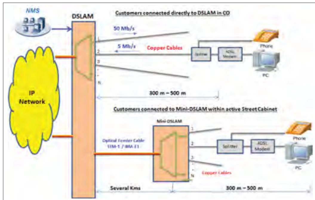
Figure 2.2 Current DSL based last-mile network
