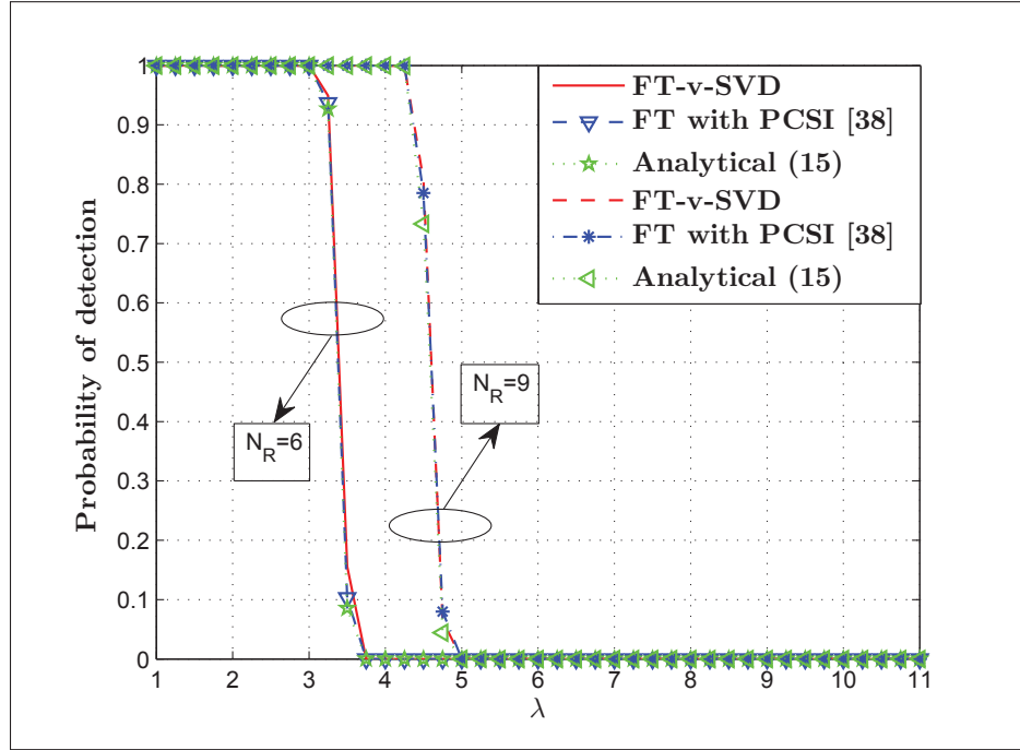
Figure 7.4 P_d versus \lambda : \gamma_{\text{snr}} = -4 dB. Note that [38] represents (Huang & Chung, 2013a) and (15) stands for (7.15)
