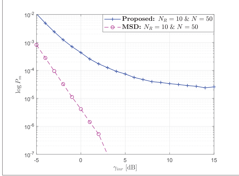
Figure 4.5 P_m versus \gamma_{inr} : P_f = 0.01 and 10^7 channel realizations
