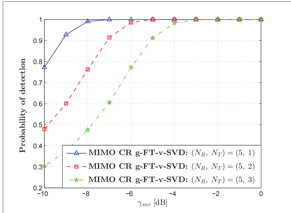
Figure 7.20 P_d versus \gamma_{snr} : P_f = 0.1 and 10^4 realizations
