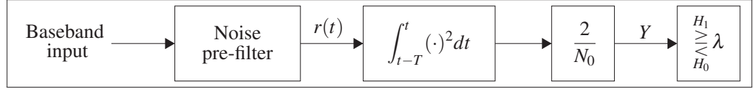
Figure 3.1 The investigated energy-based RFI detector
