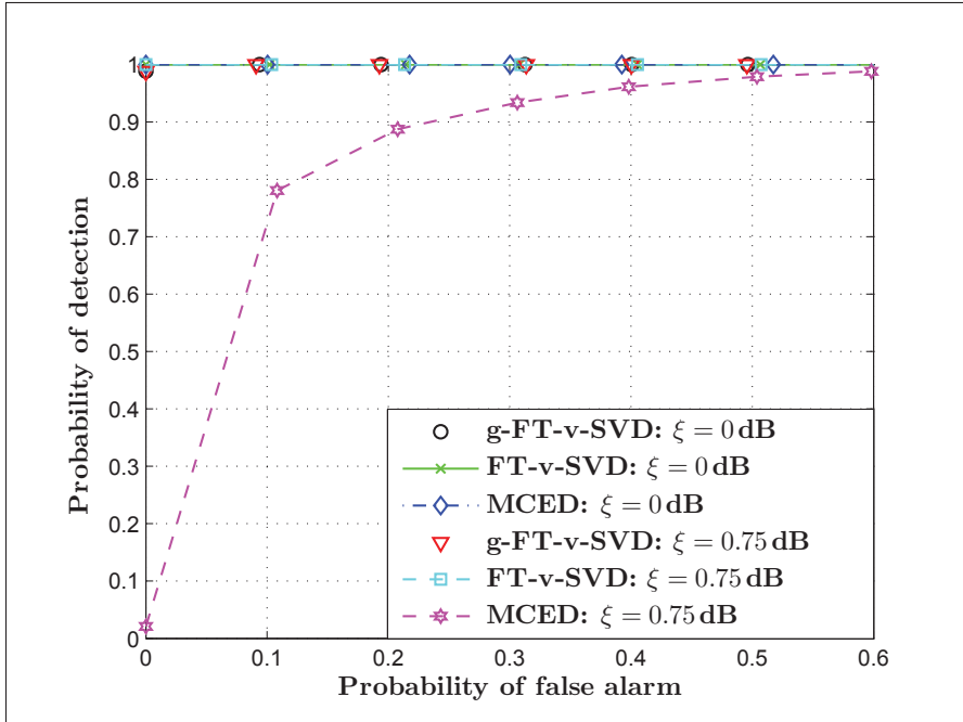
Figure 7.22 P_d versus P_f : (N(\equiv \tilde{N}W), \gamma_{snr}) = (300, -6 \text{ dB}) , and 10^5 realizations
