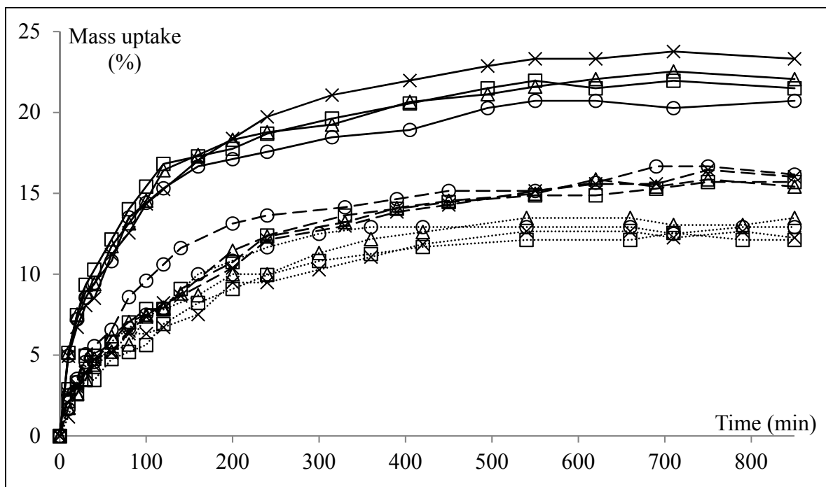
Figure 4-3. Mass uptake of NBR/P and RCN for different nClays in different solvents at 23°C. Line styles refer to: (···) isopropanol, (---) ethanol and (—) methanol
