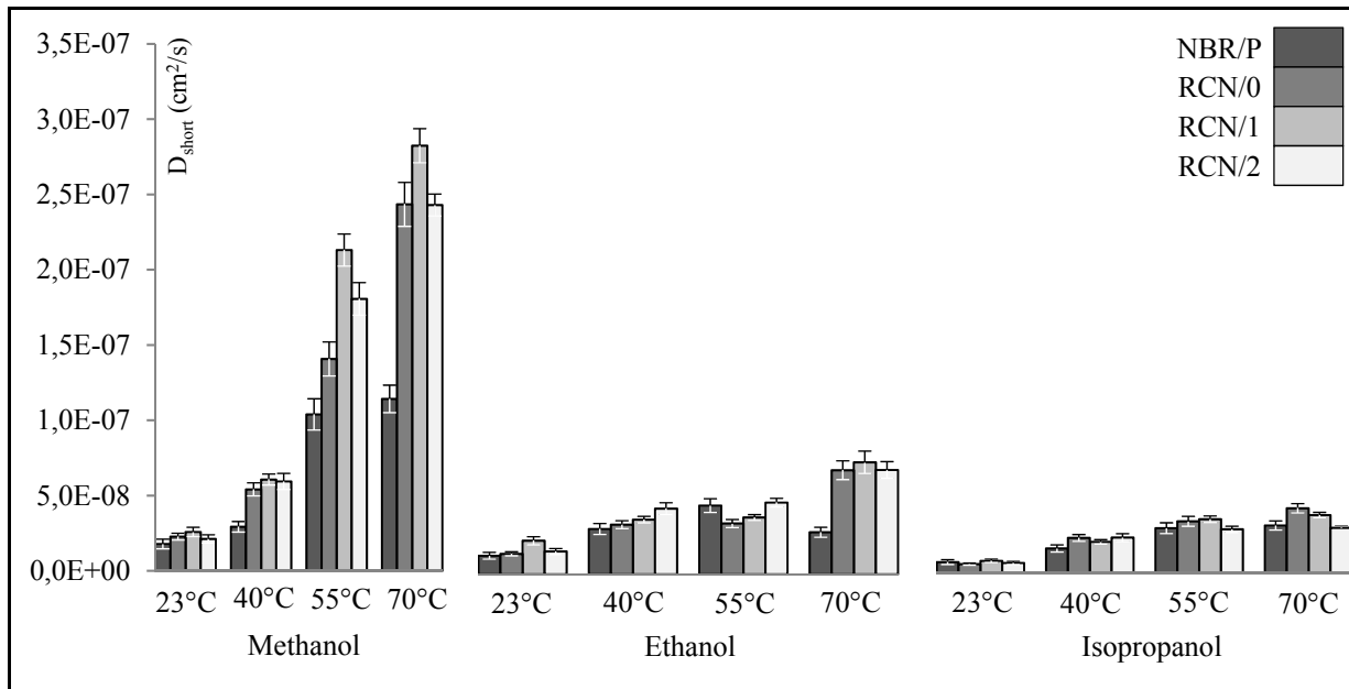
Figure 4-8. Diffusion coefficients of methanol, ethanol and isopropanol in NBR/P, RCN/0, RCN/1 and RCN/2 at 23°C, 40°C, 55°C and 70°C
