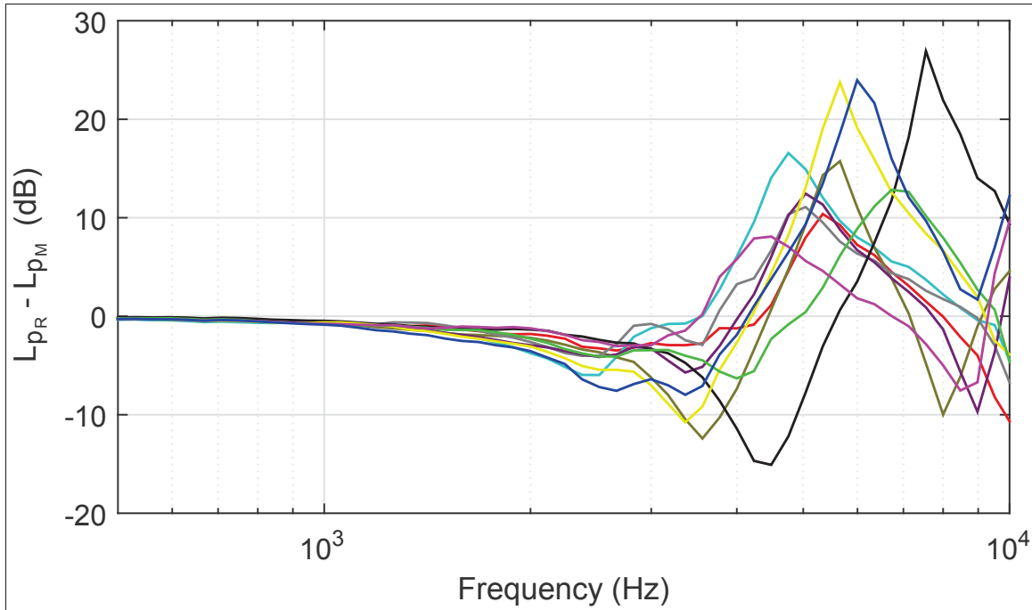
Figure 3.22 Response curves measured on the 10 participants wearing the developed dosimetric earpiece under approximate diffuse-field conditions, in 1/12^{\text{th}} octave band frequencies. Overall, the expected spectrum maximum is clearly visible for all participants, and occurs between 4.5 and 7.5 kHz
