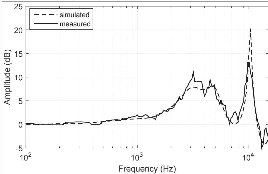
Figure 3.2 Sound pressure transformation from ear canal entrance to eardrum compared between model predictions and real-ear measurements for ear canal E of known dimensions (Fig. 3.1). Results are presented in 1/24^{\text{th}} octave band frequencies, and align well up to 10 kHz. The first and second peaks represent the first and second natural resonances of the ear canal, and are typical of the human ear. Model predictions overestimate the amplitude of the second resonance
