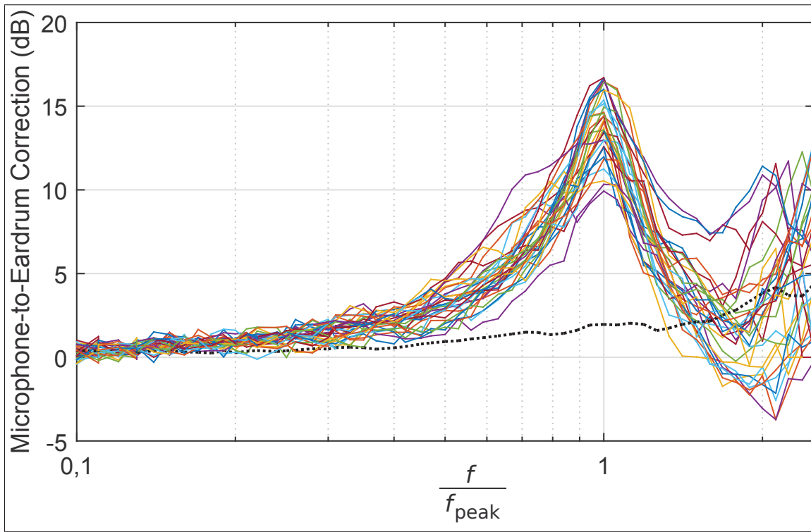
Figure 3.10 MECs measured on 10 participants at 8, 10, and 12 mm from the ECE. For a shape comparison, the MECs are presented in 1/12^{\text{th}} octave band frequencies and positioned on the x -axis to make all maxima coincide. The black dotted line indicates the standard deviation ( N=30 )
