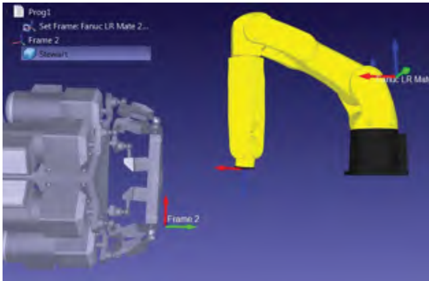
Figure 2.8 A first try to place hexapod in Fanuc's workspace. The singularity of Fanuc is not considered and also it is not applicable regarding the constraint of being on the same level as Fanuc.
