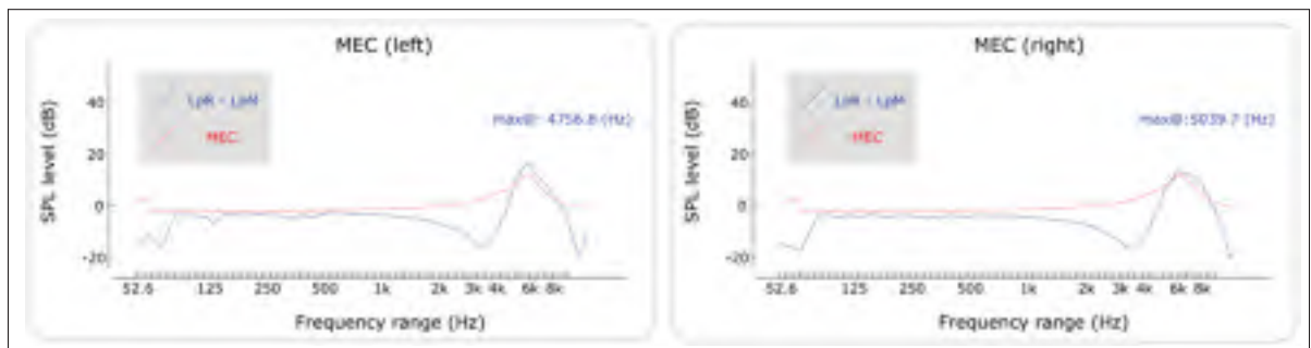
Figure 3.25 Examples of MEC curves obtained on a given subject wearing the OED
