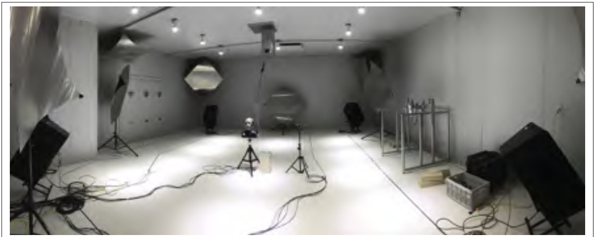
Figure 4.3 Example of the reverberant room used for tests with the same earpieces
