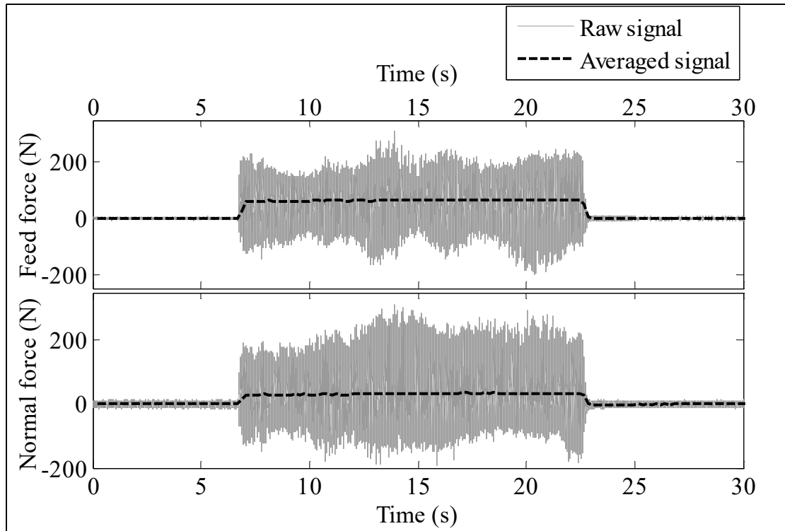
Figure 3.7 Forces signals
